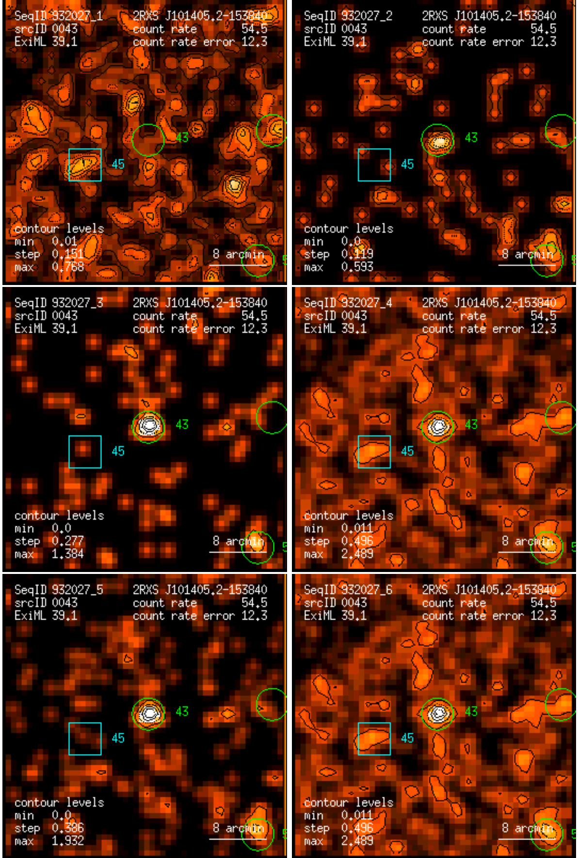
Figure 43: RASS 932027: detection 0043: band rate images, Gaussian filter: (1) PSPC channels 11 – 41, (2) 52 – 90, (3) 91 – 201, (4) 11 – 235, (5) 52 – 201, (6) 11 – 201. Broad band rates in counts/ks. Band rate contour levels in counts/ks/arcmin 2 .
