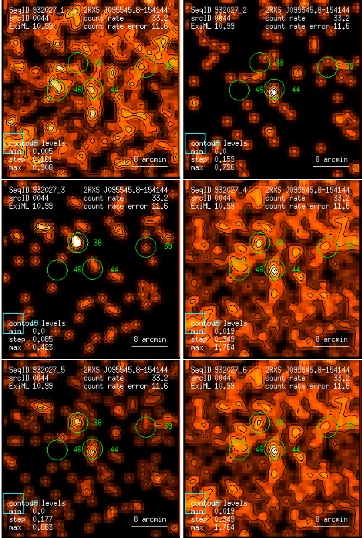
Figure 44: RASS 932027: detection 0044: band rate images, Gaussian filter: (1) PSPC channels 11 – 41, (2) 52 – 90, (3) 91 – 201, (4) 11 – 235, (5) 52 – 201, (6) 11 – 201. Broad band rates in counts/ks. Band rate contour levels in counts/ks/arcmin 2 .
