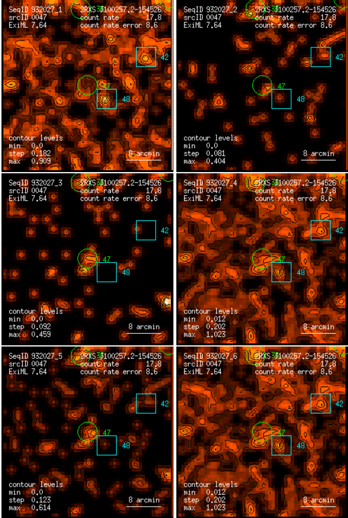
Figure 47: RASS 932027: detection 0047: band rate images, Gaussian filter: (1) PSPC channels 11 – 41, (2) 52 – 90, (3) 91 – 201, (4) 11 – 235, (5) 52 – 201, (6) 11 – 201. Broad band rates in counts/ks. Band rate contour levels in counts/ks/arcmin 2 .
