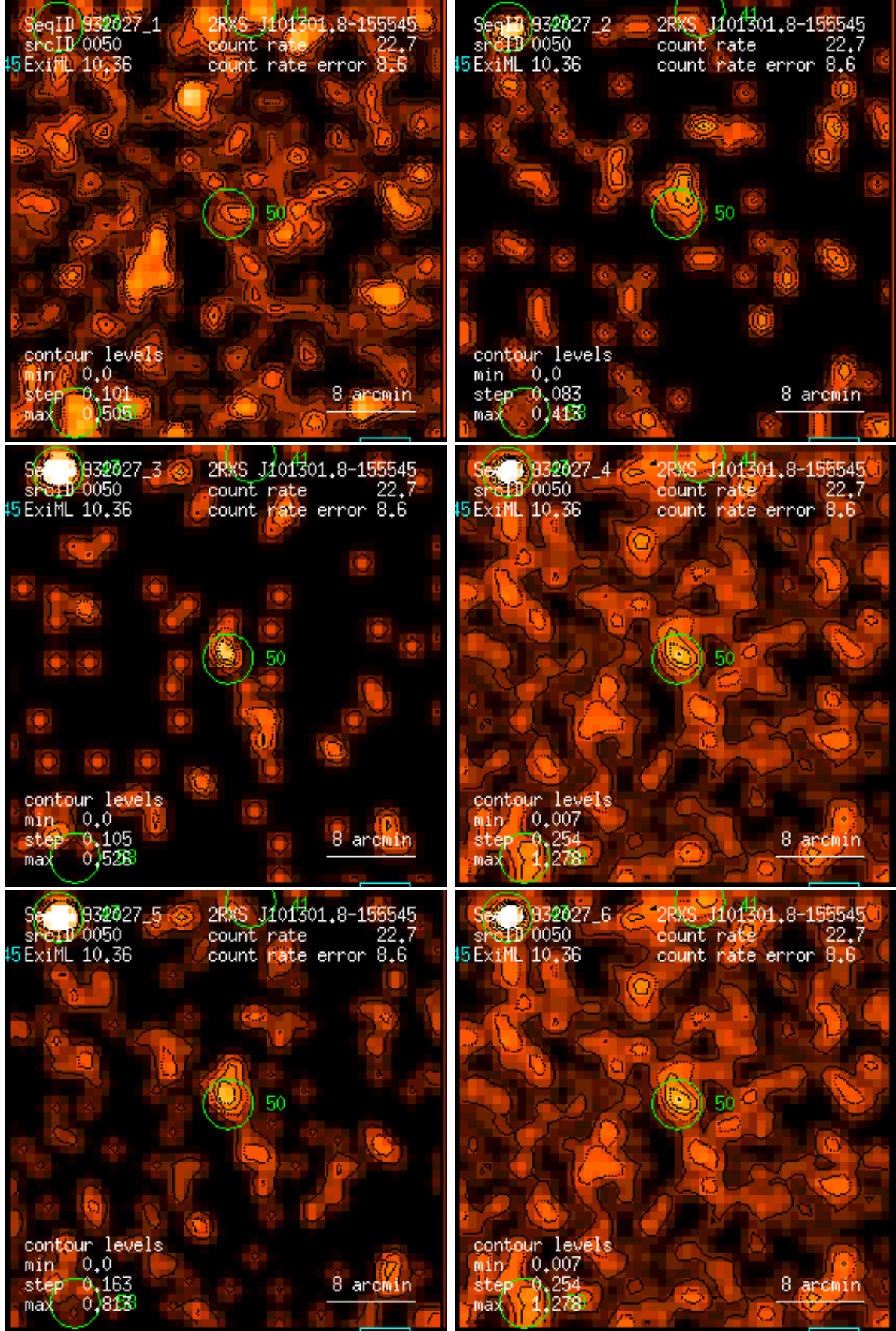
Figure 50: RASS 932027: detection 0050: band rate images, Gaussian filter: (1) PSPC channels 11 – 41, (2) 52 – 90, (3) 91 – 201, (4) 11 – 235, (5) 52 – 201, (6) 11 – 201. Broad band rates in counts/ks. Band rate contour levels in counts/ks/arcmin 2 .
