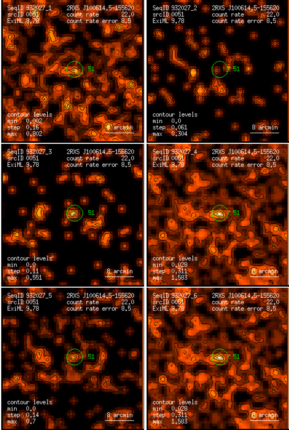
Figure 51: RASS 932027: detection 0051: band rate images, Gaussian filter: (1) PSPC channels 11 – 41, (2) 52 – 90, (3) 91 – 201, (4) 11 – 235, (5) 52 – 201, (6) 11 – 201. Broad band rates in counts/ks. Band rate contour levels in counts/ks/arcmin 2 .
