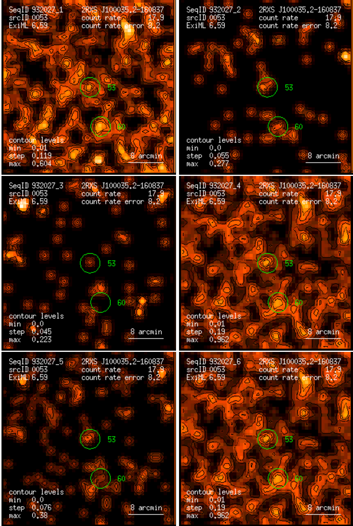
Figure 53: RASS 932027: detection 0053: band rate images, Gaussian filter: (1) PSPC channels 11 – 41, (2) 52 – 90, (3) 91 – 201, (4) 11 – 235, (5) 52 – 201, (6) 11 – 201. Broad band rates in counts/ks. Band rate contour levels in counts/ks/arcmin 2 .
