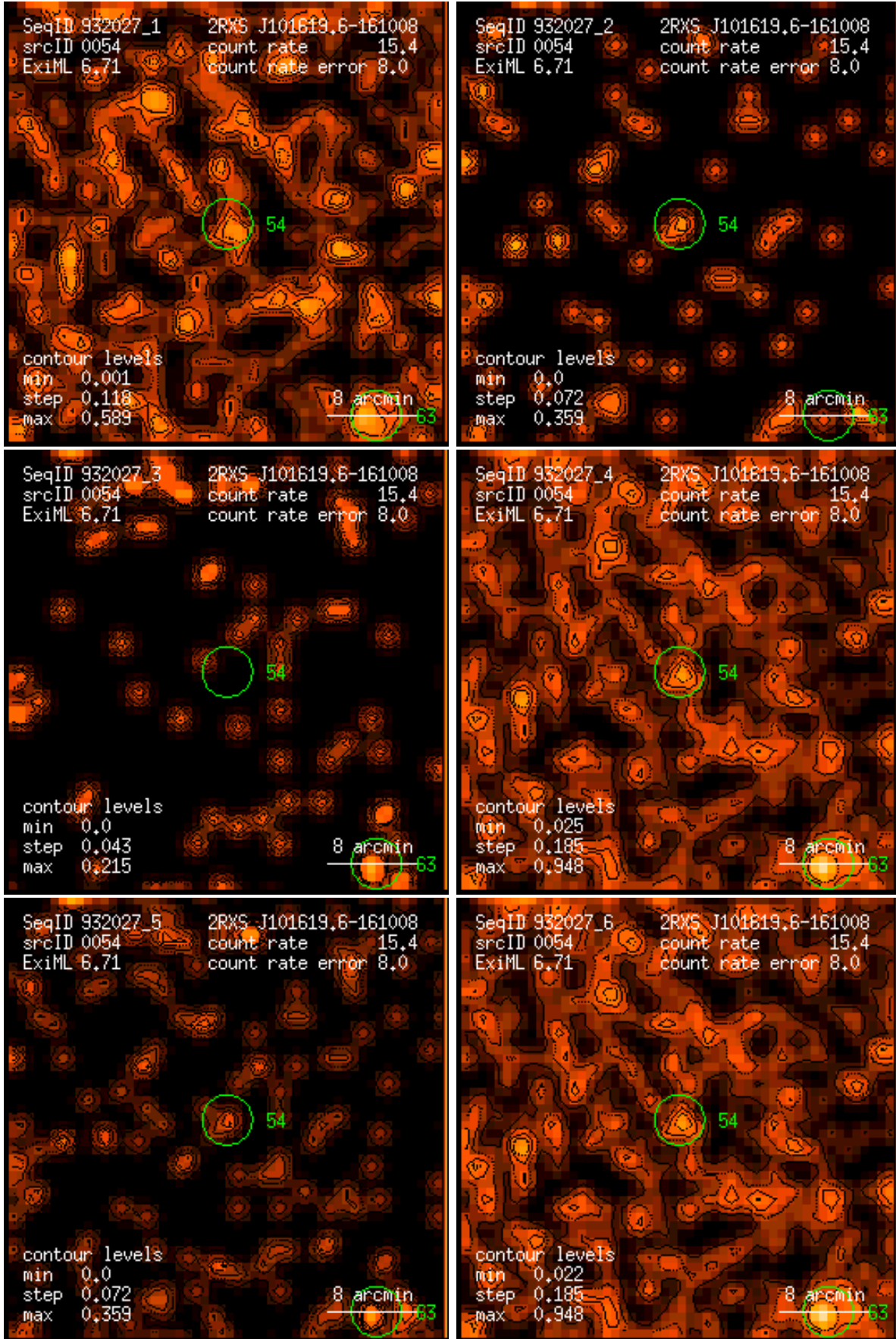
Figure 54: RASS 932027: detection 0054: band rate images, Gaussian filter: (1) PSPC channels 11 – 41, (2) 52 – 90, (3) 91 – 201, (4) 11 – 235, (5) 52 – 201, (6) 11 – 201. Broad band rates in counts/ks. Band rate contour levels in counts/ks/arcmin 2 .
