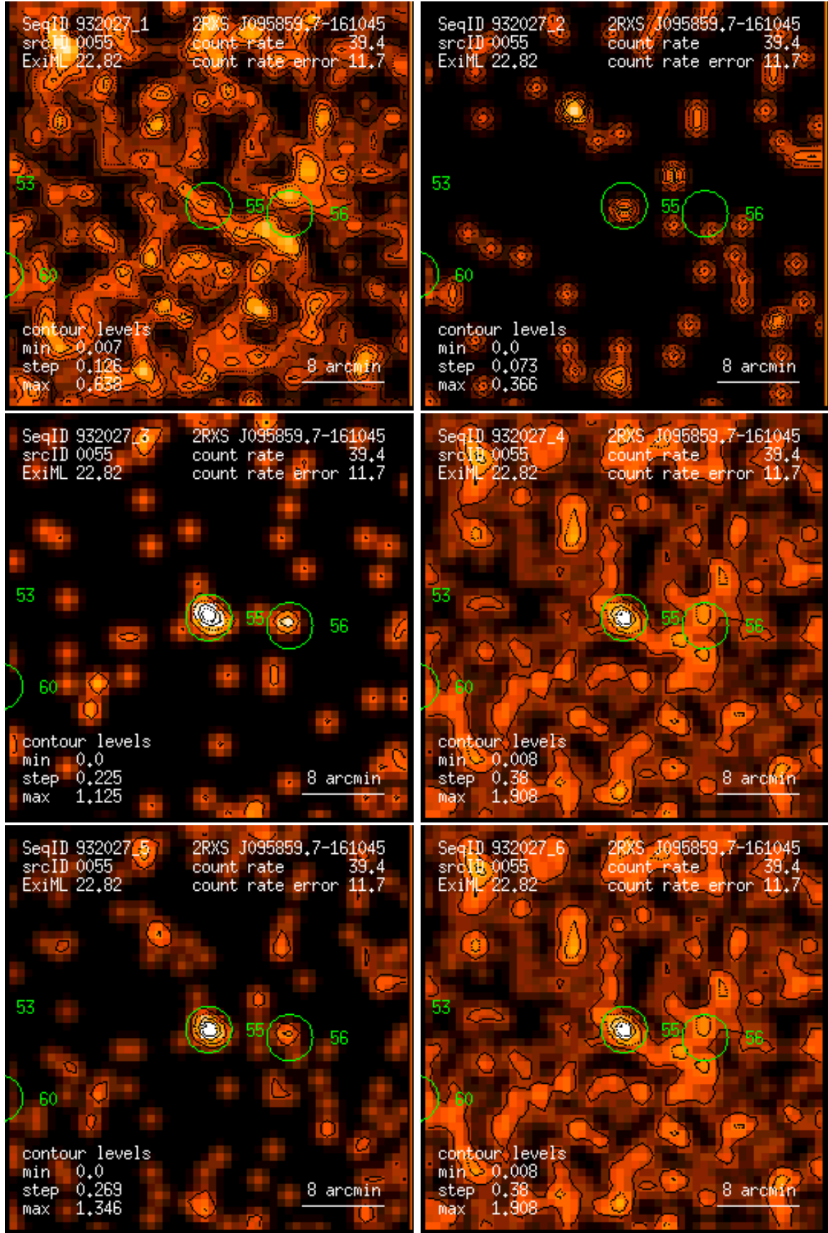
Figure 55: RASS 932027: detection 0055: band rate images, Gaussian filter: (1) PSPC channels 11 – 41, (2) 52 – 90, (3) 91 – 201, (4) 11 – 235, (5) 52 – 201, (6) 11 – 201. Broad band rates in counts/ks. Band rate contour levels in counts/ks/arcmin 2 .
