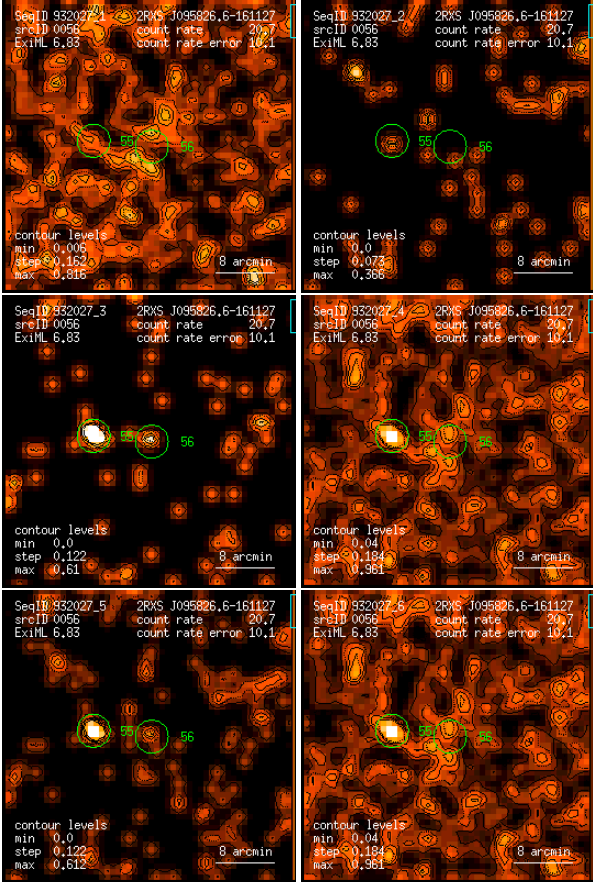
Figure 56: RASS 932027: detection 0056: band rate images, Gaussian filter: (1) PSPC channels 11 – 41, (2) 52 – 90, (3) 91 – 201, (4) 11 – 235, (5) 52 – 201, (6) 11 – 201. Broad band rates in counts/ks. Band rate contour levels in counts/ks/arcmin 2 .
