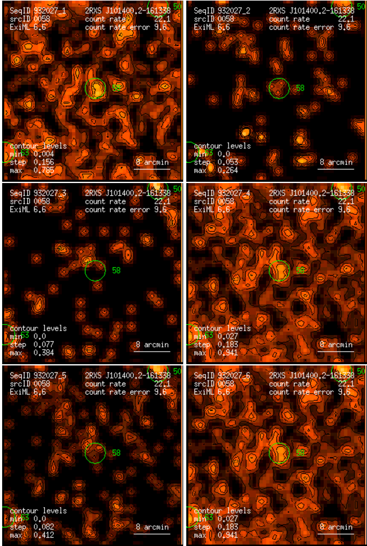
Figure 58: RASS 932027: detection 0058: band rate images, Gaussian filter: (1) PSPC channels 11 – 41, (2) 52 – 90, (3) 91 – 201, (4) 11 – 235, (5) 52 – 201, (6) 11 – 201. Broad band rates in counts/ks. Band rate contour levels in counts/ks/arcmin 2 .
