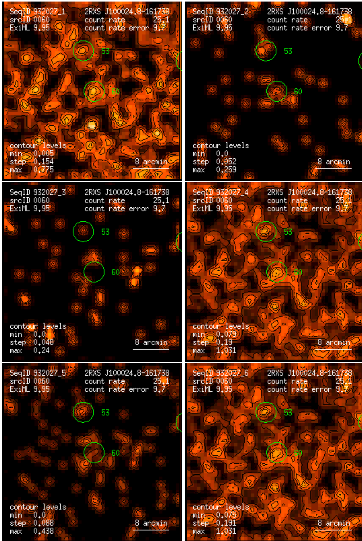
Figure 60: RASS 932027: detection 0060: band rate images, Gaussian filter: (1) PSPC channels 11 – 41, (2) 52 – 90, (3) 91 – 201, (4) 11 – 235, (5) 52 – 201, (6) 11 – 201. Broad band rates in counts/ks. Band rate contour levels in counts/ks/arcmin 2 .
