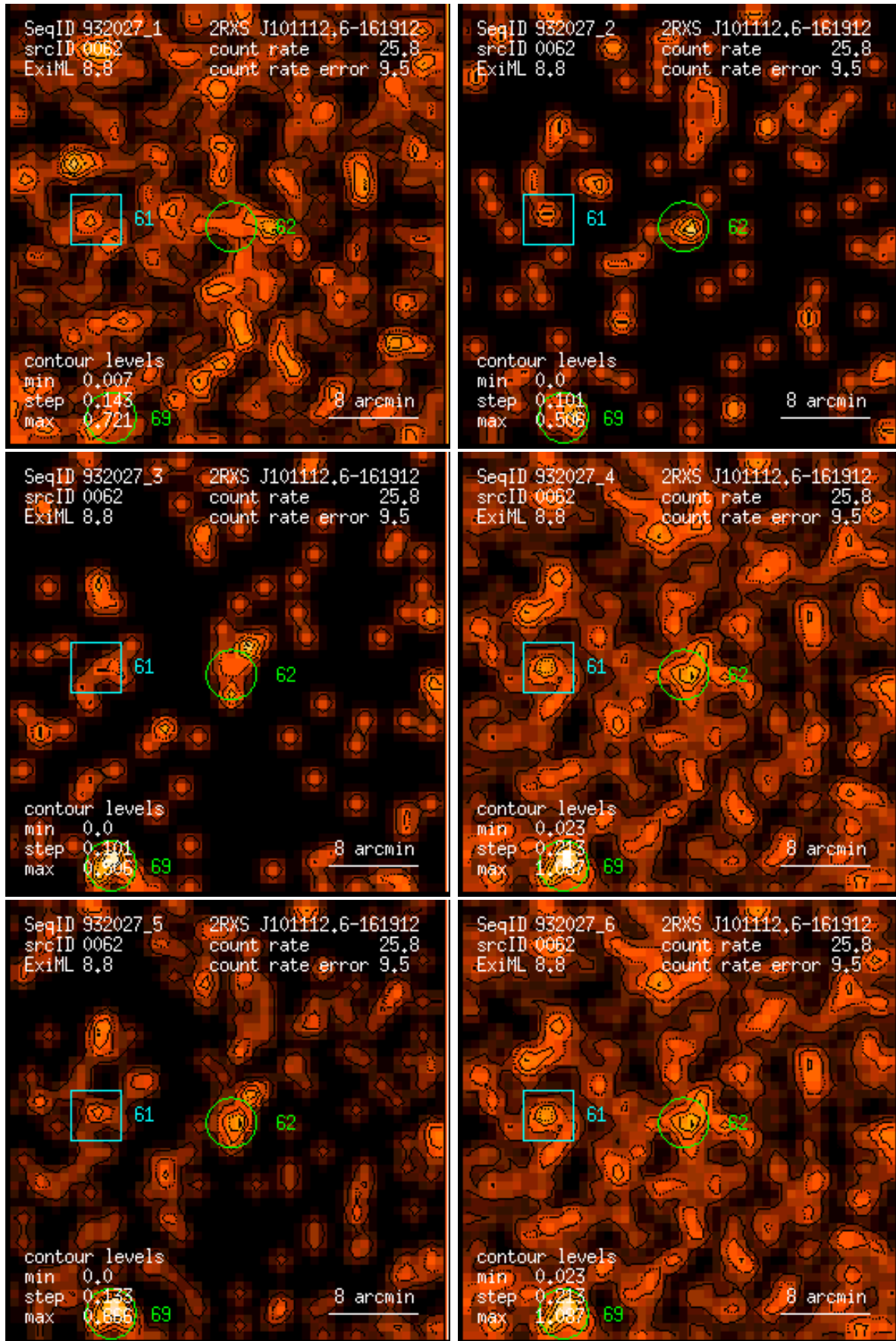
Figure 62: RASS 932027: detection 0062: band rate images, Gaussian filter: (1) PSPC channels 11 – 41, (2) 52 – 90, (3) 91 – 201, (4) 11 – 235, (5) 52 – 201, (6) 11 – 201. Broad band rates in counts/ks. Band rate contour levels in counts/ks/arcmin 2 .
