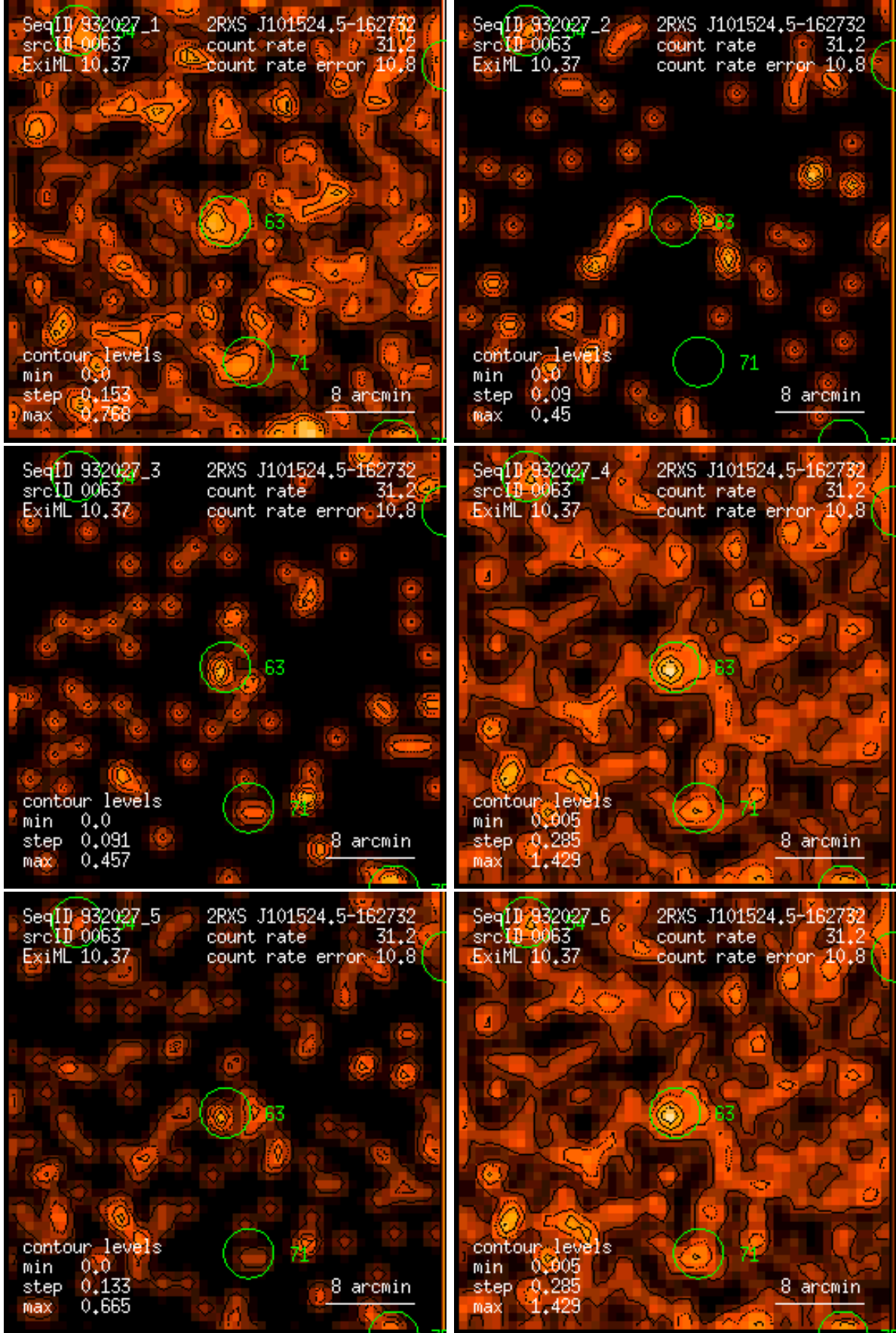
Figure 63: RASS 932027: detection 0063: band rate images, Gaussian filter: (1) PSPC channels 11 – 41, (2) 52 – 90, (3) 91 – 201, (4) 11 – 235, (5) 52 – 201, (6) 11 – 201. Broad band rates in counts/ks. Band rate contour levels in counts/ks/arcmin 2 .
