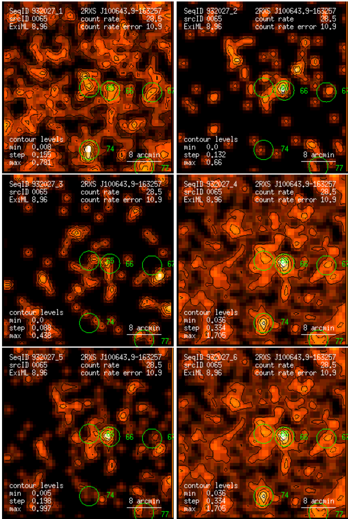
Figure 65: RASS 932027: detection 0065: band rate images, Gaussian filter: (1) PSPC channels 11 – 41, (2) 52 – 90, (3) 91 – 201, (4) 11 – 235, (5) 52 – 201, (6) 11 – 201. Broad band rates in counts/ks. Band rate contour levels in counts/ks/arcmin 2 .
