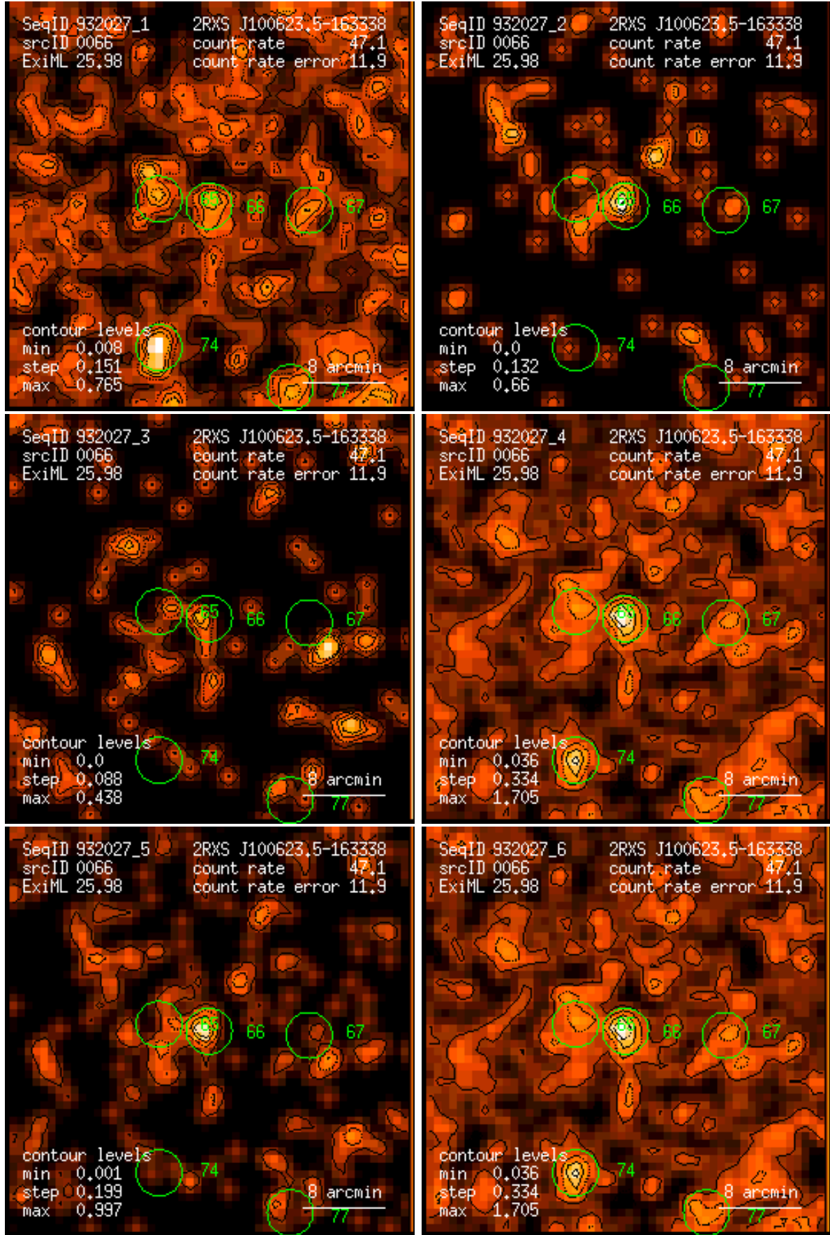
Figure 66: RASS 932027: detection 0066: band rate images, Gaussian filter: (1) PSPC channels 11 – 41, (2) 52 – 90, (3) 91 – 201, (4) 11 – 235, (5) 52 – 201, (6) 11 – 201. Broad band rates in counts/ks. Band rate contour levels in counts/ks/arcmin 2 .
