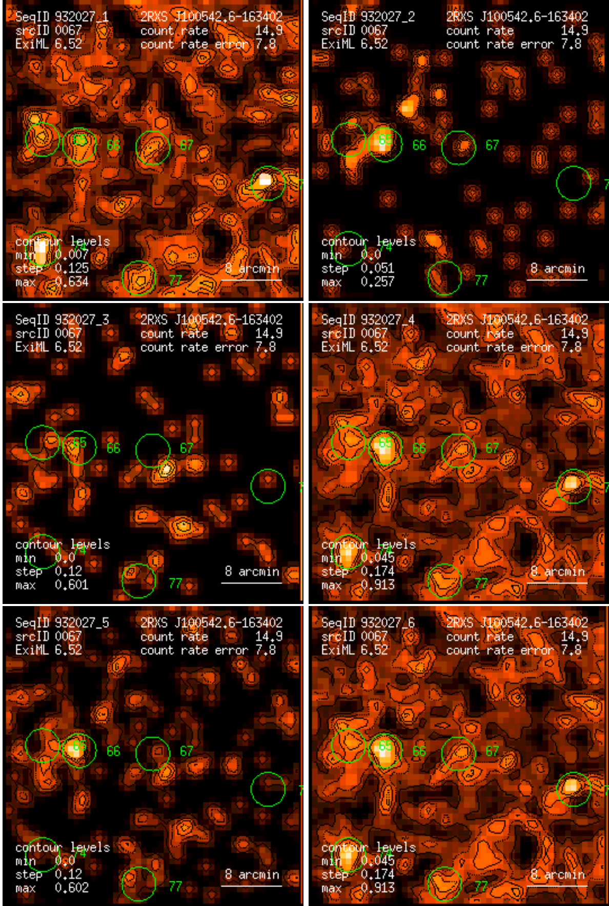
Figure 67: RASS 932027: detection 0067: band rate images, Gaussian filter: (1) PSPC channels 11 – 41, (2) 52 – 90, (3) 91 – 201, (4) 11 – 235, (5) 52 – 201, (6) 11 – 201. Broad band rates in counts/ks. Band rate contour levels in counts/ks/arcmin 2 .
