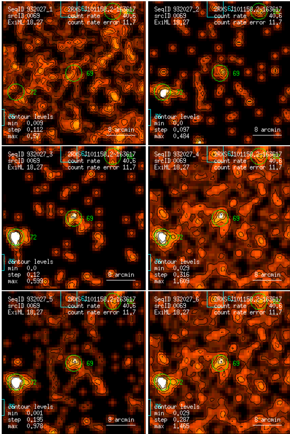
Figure 69: RASS 932027: detection 0069: band rate images, Gaussian filter: (1) PSPC channels 11 – 41, (2) 52 – 90, (3) 91 – 201, (4) 11 – 235, (5) 52 – 201, (6) 11 – 201. Broad band rates in counts/ks. Band rate contour levels in counts/ks/arcmin 2 .
