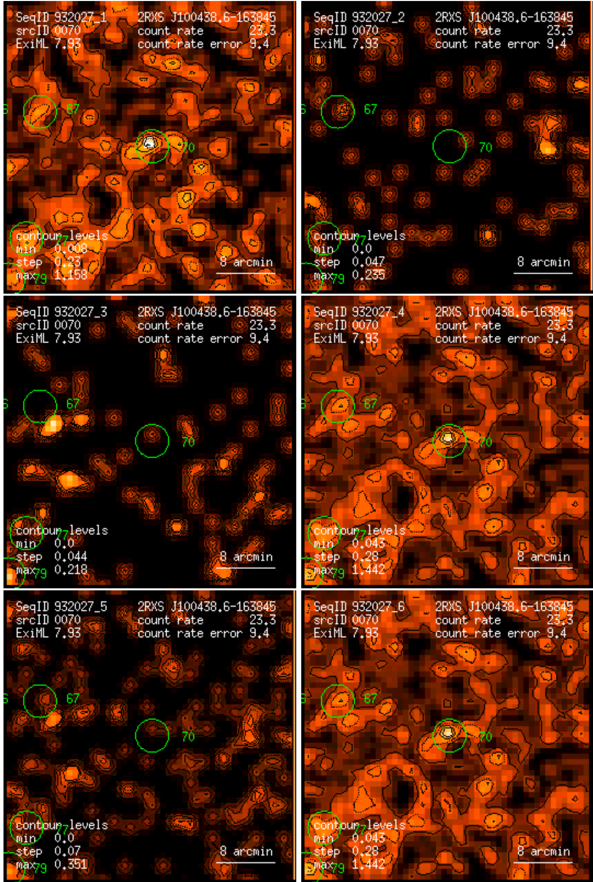
Figure 70: RASS 932027: detection 0070: band rate images, Gaussian filter: (1) PSPC channels 11 – 41, (2) 52 – 90, (3) 91 – 201, (4) 11 – 235, (5) 52 – 201, (6) 11 – 201. Broad band rates in counts/ks. Band rate contour levels in counts/ks/arcmin 2 .
