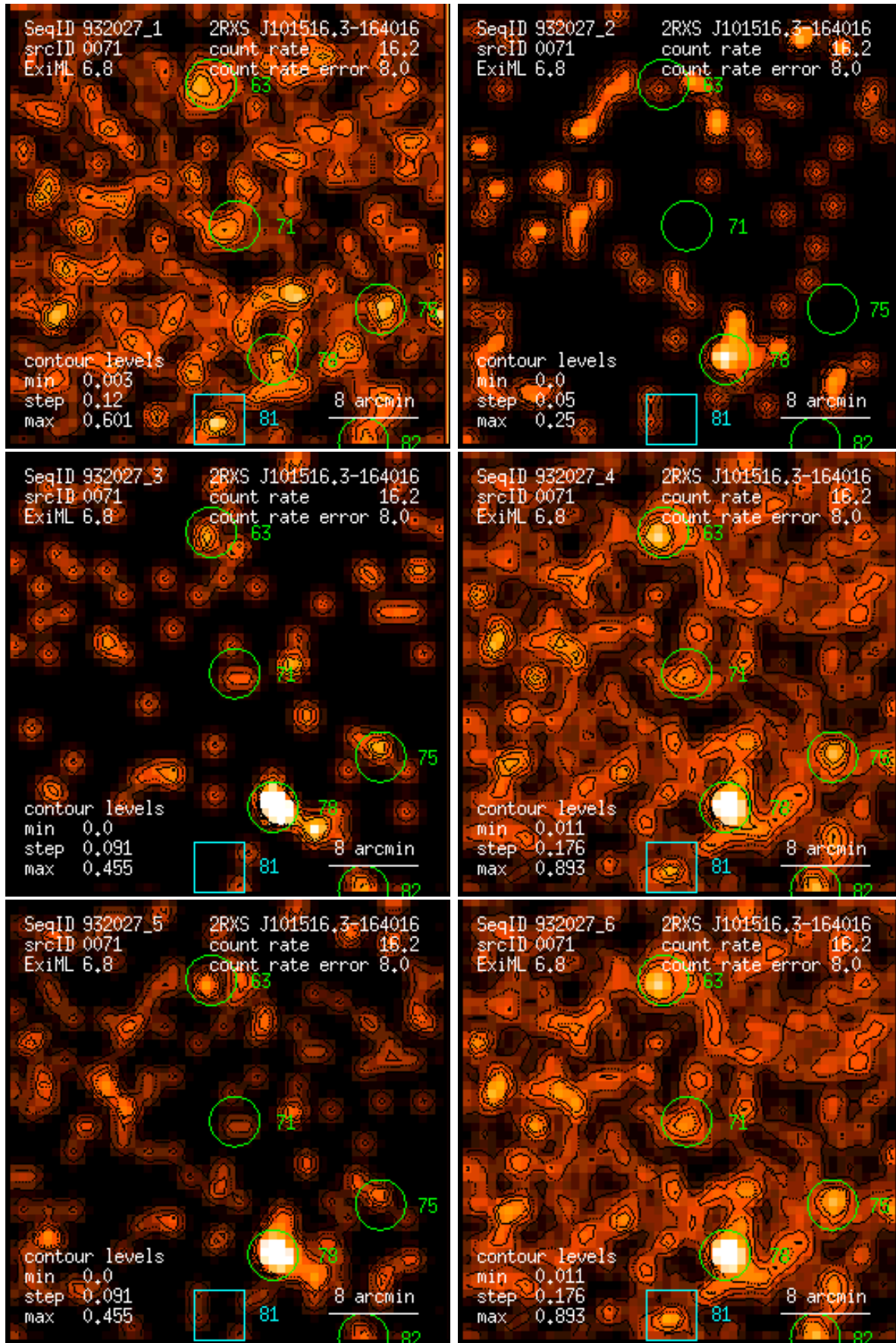
Figure 71: RASS 932027: detection 0071: band rate images, Gaussian filter: (1) PSPC channels 11 – 41, (2) 52 – 90, (3) 91 – 201, (4) 11 – 235, (5) 52 – 201, (6) 11 – 201. Broad band rates in counts/ks. Band rate contour levels in counts/ks/arcmin 2 .
