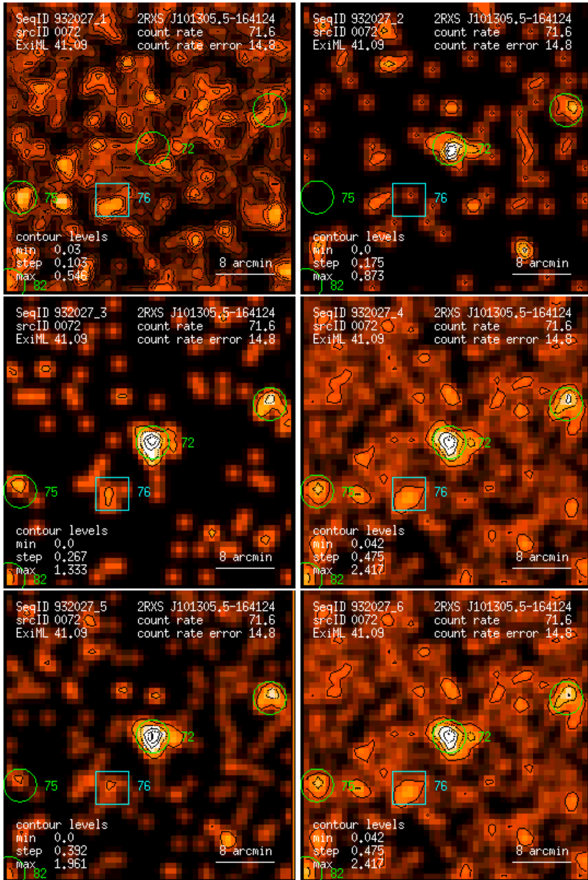
Figure 72: RASS 932027: detection 0072: band rate images, Gaussian filter: (1) PSPC channels 11 – 41, (2) 52 – 90, (3) 91 – 201, (4) 11 – 235, (5) 52 – 201, (6) 11 – 201. Broad band rates in counts/ks. Band rate contour levels in counts/ks/arcmin 2 .
