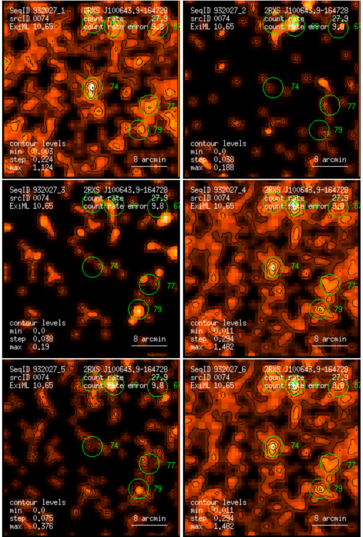
Figure 74: RASS 932027: detection 0074: band rate images, Gaussian filter: (1) PSPC channels 11 – 41, (2) 52 – 90, (3) 91 – 201, (4) 11 – 235, (5) 52 – 201, (6) 11 – 201. Broad band rates in counts/ks. Band rate contour levels in counts/ks/arcmin 2 .
