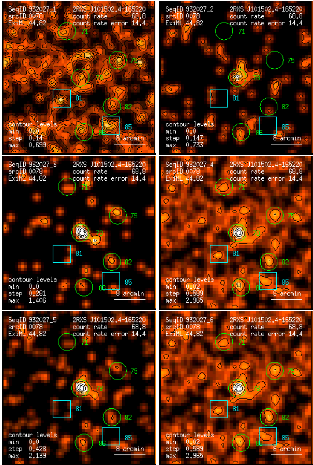
Figure 78: RASS 932027: detection 0078: band rate images, Gaussian filter: (1) PSPC channels 11 – 41, (2) 52 – 90, (3) 91 – 201, (4) 11 – 235, (5) 52 – 201, (6) 11 – 201. Broad band rates in counts/ks. Band rate contour levels in counts/ks/arcmin 2 .
