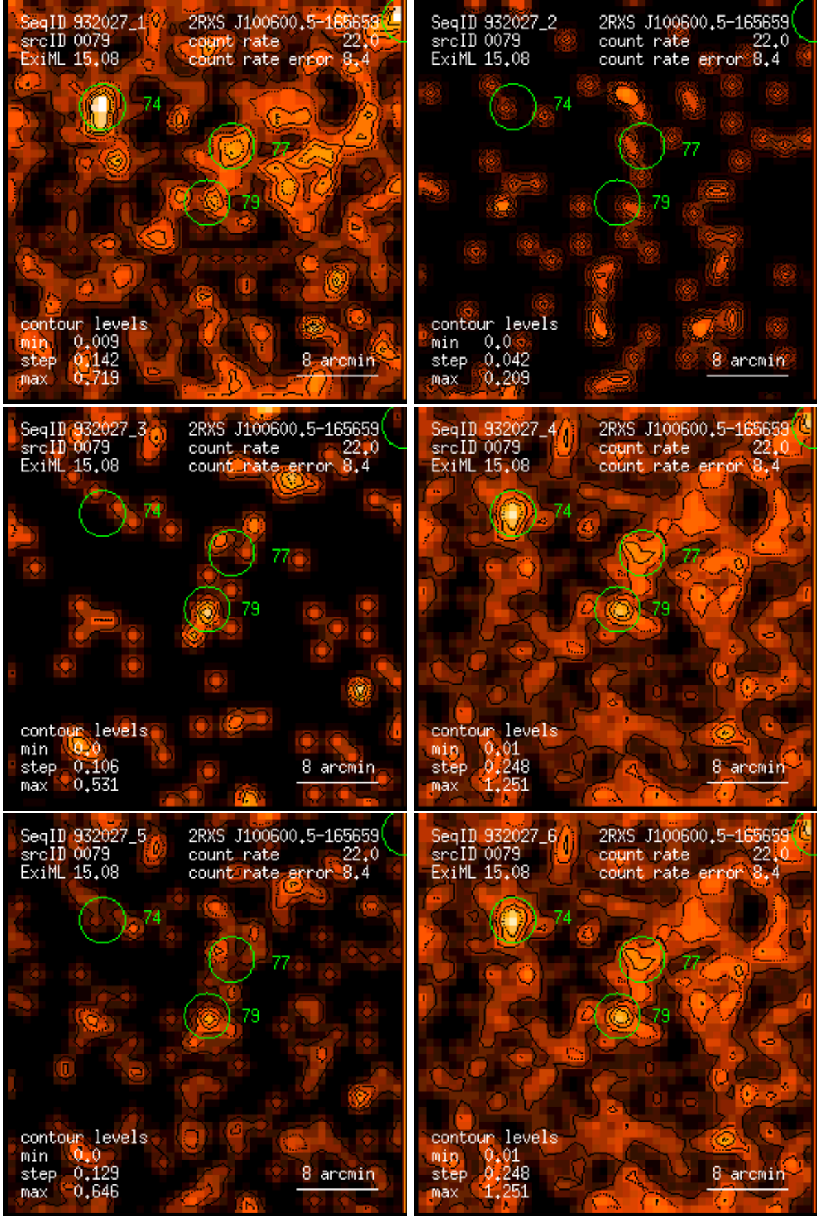
Figure 79: RASS 932027: detection 0079: band rate images, Gaussian filter: (1) PSPC channels 11 – 41, (2) 52 – 90, (3) 91 – 201, (4) 11 – 235, (5) 52 – 201, (6) 11 – 201. Broad band rates in counts/ks. Band rate contour levels in counts/ks/arcmin 2 .
