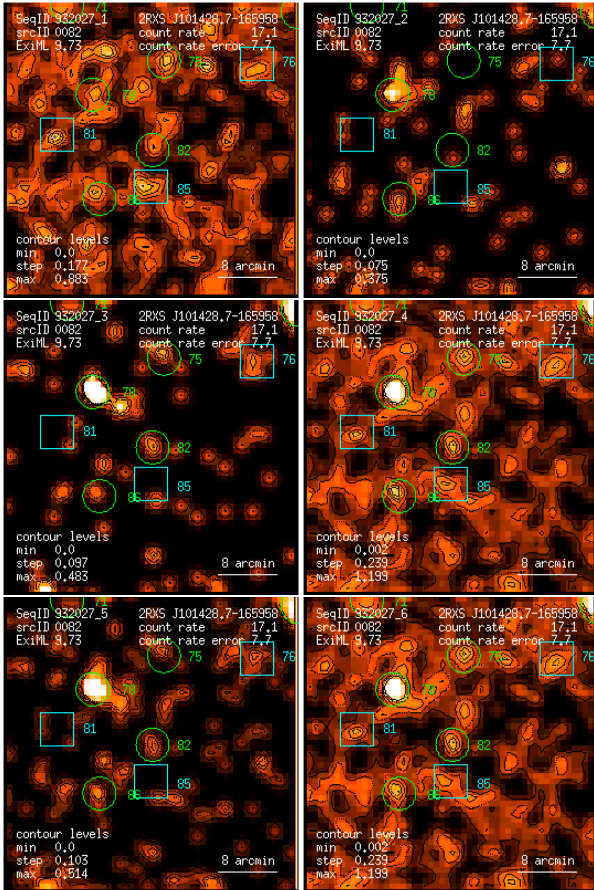
Figure 82: RASS 932027: detection 0082: band rate images, Gaussian filter: (1) PSPC channels 11 – 41, (2) 52 – 90, (3) 91 – 201, (4) 11 – 235, (5) 52 – 201, (6) 11 – 201. Broad band rates in counts/ks. Band rate contour levels in counts/ks/arcmin 2 .
