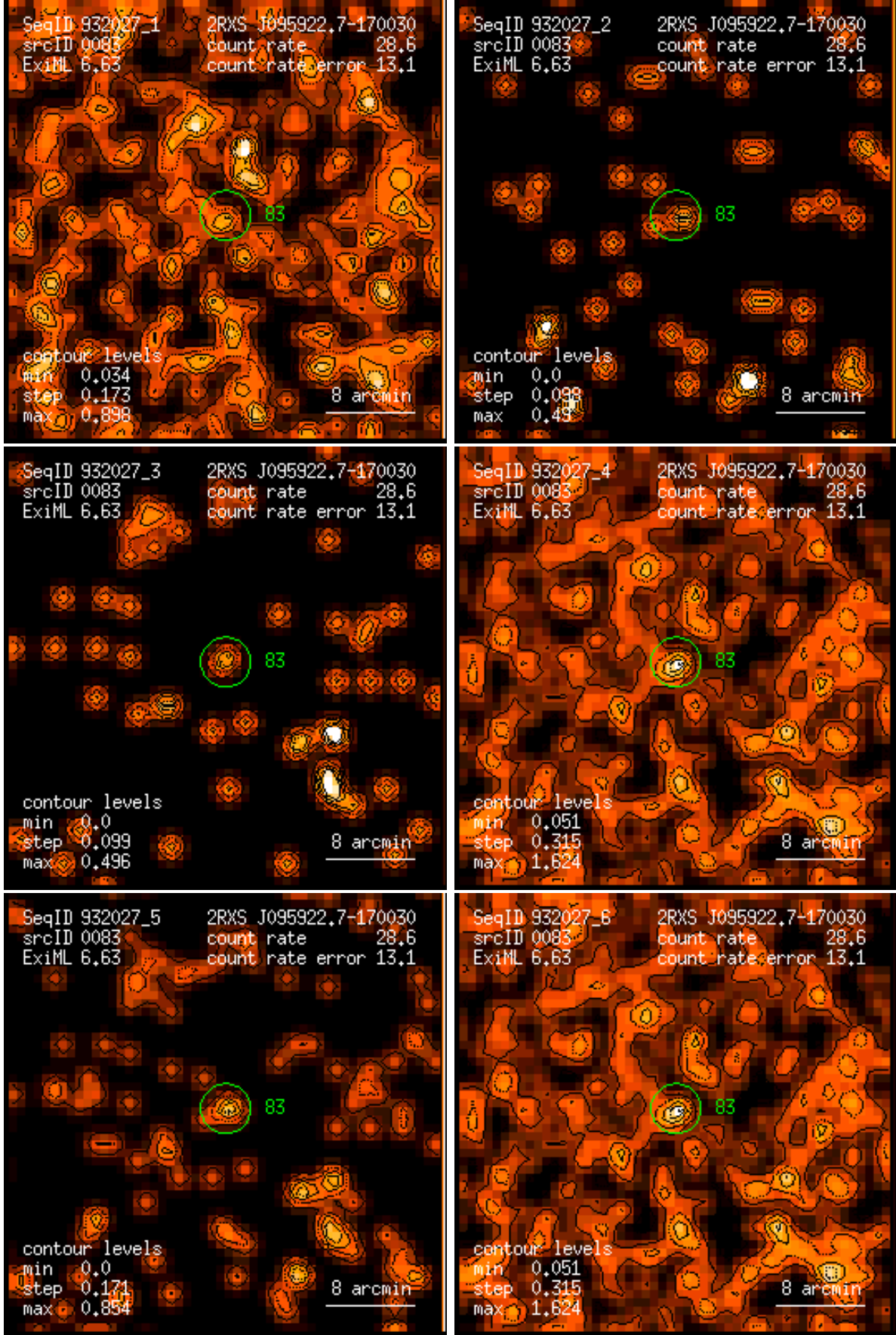
Figure 83: RASS 932027: detection 0083: band rate images, Gaussian filter: (1) PSPC channels 11 – 41, (2) 52 – 90, (3) 91 – 201, (4) 11 – 235, (5) 52 – 201, (6) 11 – 201. Broad band rates in counts/ks. Band rate contour levels in counts/ks/arcmin 2 .
