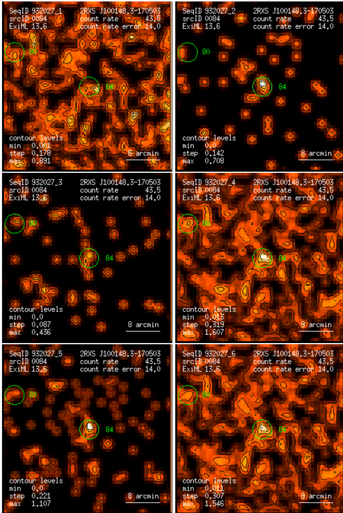
Figure 84: RASS 932027: detection 0084: band rate images, Gaussian filter: (1) PSPC channels 11 – 41, (2) 52 – 90, (3) 91 – 201, (4) 11 – 235, (5) 52 – 201, (6) 11 – 201. Broad band rates in counts/ks. Band rate contour levels in counts/ks/arcmin 2 .
