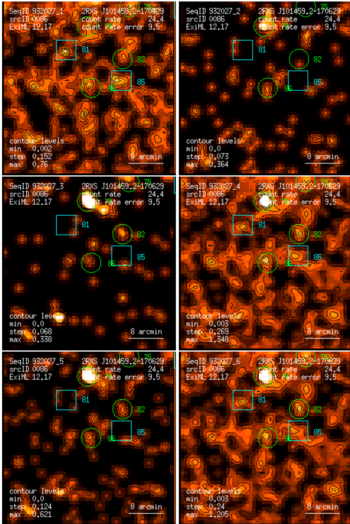
Figure 86: RASS 932027: detection 0086: band rate images, Gaussian filter: (1) PSPC channels 11 – 41, (2) 52 – 90, (3) 91 – 201, (4) 11 – 235, (5) 52 – 201, (6) 11 – 201. Broad band rates in counts/ks. Band rate contour levels in counts/ks/arcmin 2 .
