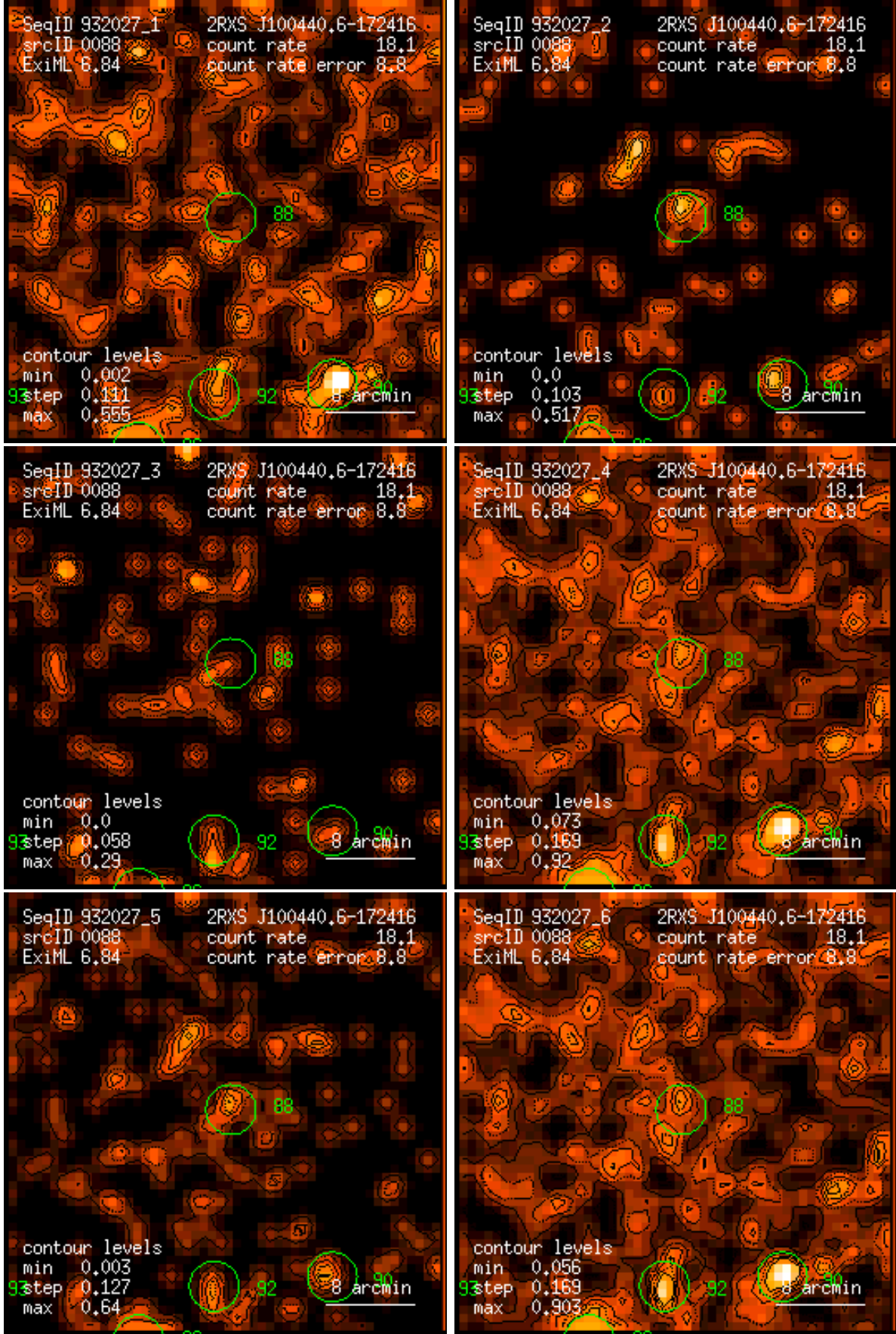
Figure 88: RASS 932027: detection 0088: band rate images, Gaussian filter: (1) PSPC channels 11 – 41, (2) 52 – 90, (3) 91 – 201, (4) 11 – 235, (5) 52 – 201, (6) 11 – 201. Broad band rates in counts/ks. Band rate contour levels in counts/ks/arcmin 2 .
