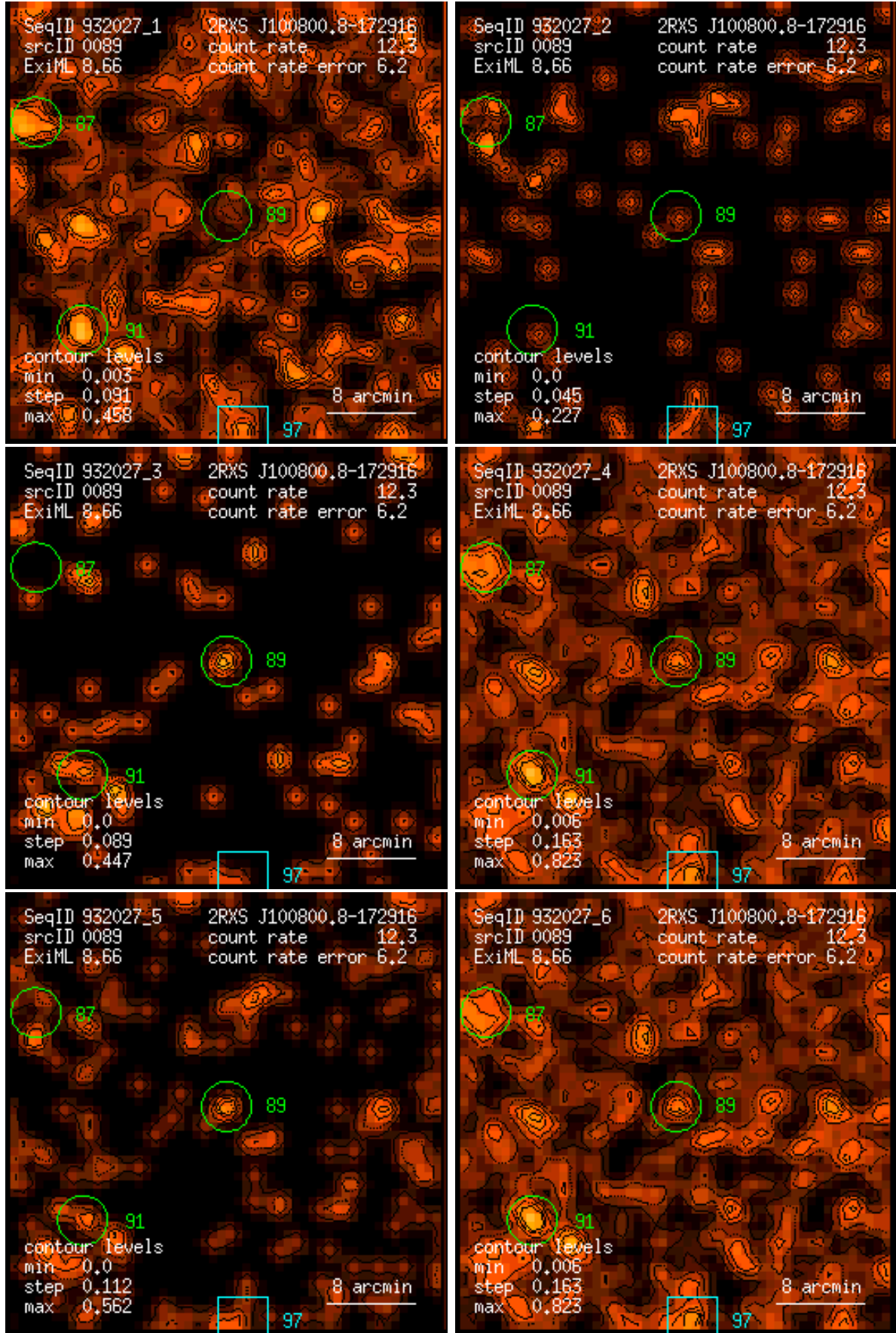
Figure 89: RASS 932027: detection 0089: band rate images, Gaussian filter: (1) PSPC channels 11 – 41, (2) 52 – 90, (3) 91 – 201, (4) 11 – 235, (5) 52 – 201, (6) 11 – 201. Broad band rates in counts/ks. Band rate contour levels in counts/ks/arcmin 2 .
