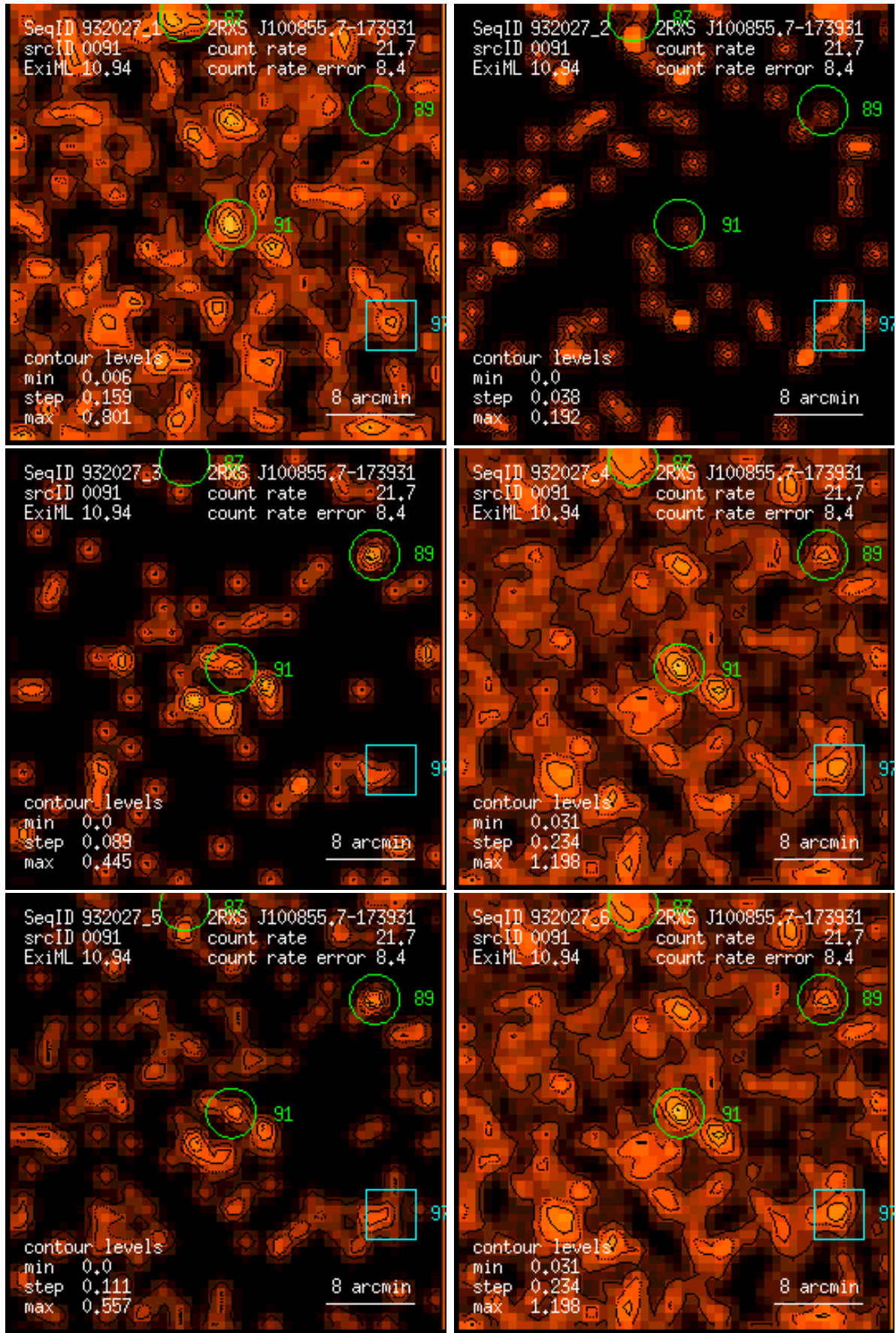
Figure 91: RASS 932027: detection 0091: band rate images, Gaussian filter: (1) PSPC channels 11 – 41, (2) 52 – 90, (3) 91 – 201, (4) 11 – 235, (5) 52 – 201, (6) 11 – 201. Broad band rates in counts/ks. Band rate contour levels in counts/ks/arcmin 2 .
