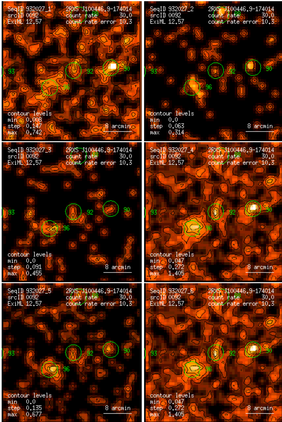
Figure 92: RASS 932027: detection 0092: band rate images, Gaussian filter: (1) PSPC channels 11 – 41, (2) 52 – 90, (3) 91 – 201, (4) 11 – 235, (5) 52 – 201, (6) 11 – 201. Broad band rates in counts/ks. Band rate contour levels in counts/ks/arcmin 2 .
