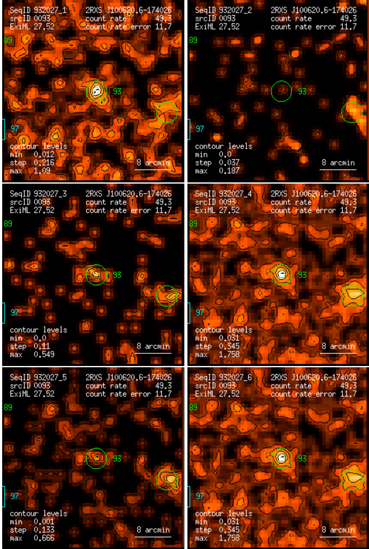
Figure 93: RASS 932027: detection 0093: band rate images, Gaussian filter: (1) PSPC channels 11 – 41, (2) 52 – 90, (3) 91 – 201, (4) 11 – 235, (5) 52 – 201, (6) 11 – 201. Broad band rates in counts/ks. Band rate contour levels in counts/ks/arcmin 2 .
