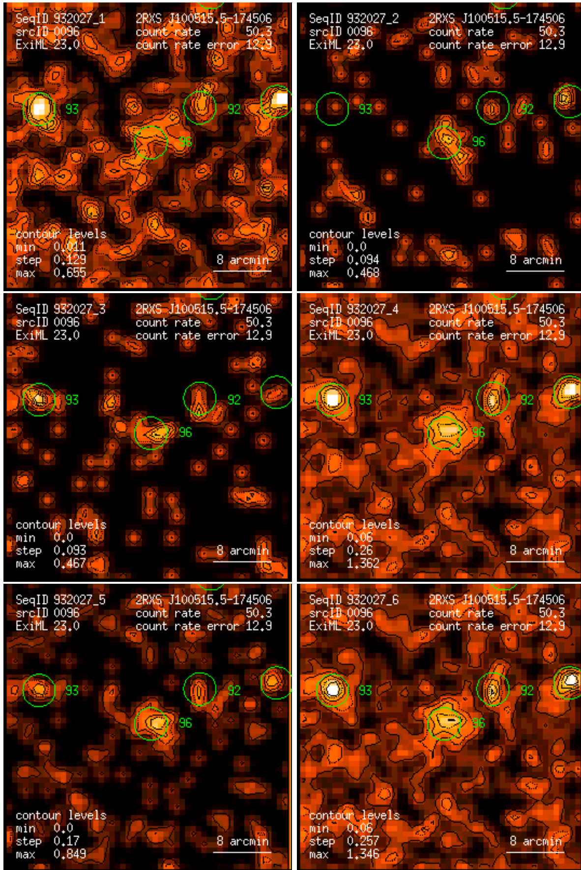
Figure 96: RASS 932027: detection 0096: band rate images, Gaussian filter: (1) PSPC channels 11 – 41, (2) 52 – 90, (3) 91 – 201, (4) 11 – 235, (5) 52 – 201, (6) 11 – 201. Broad band rates in counts/ks. Band rate contour levels in counts/ks/arcmin 2 .
