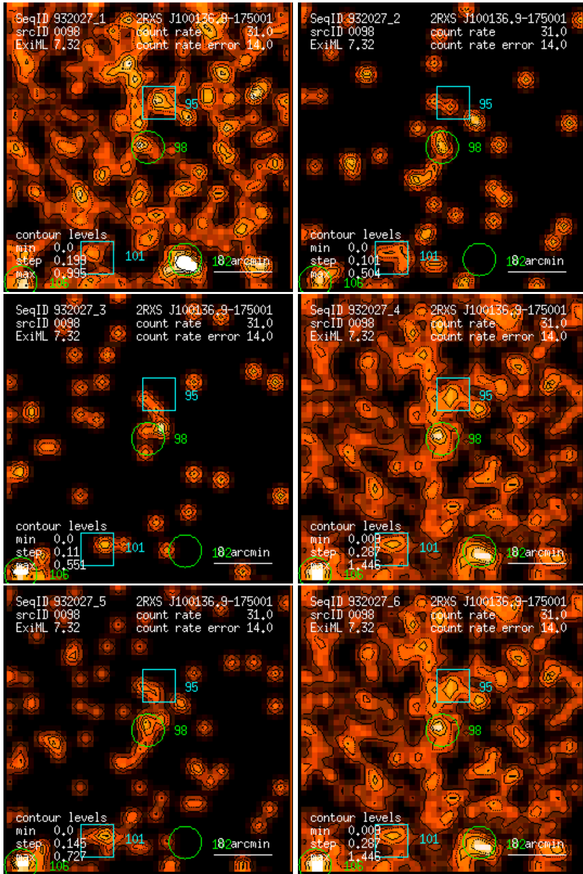
Figure 98: RASS 932027: detection 0098: band rate images, Gaussian filter: (1) PSPC channels 11 – 41, (2) 52 – 90, (3) 91 – 201, (4) 11 – 235, (5) 52 – 201, (6) 11 – 201. Broad band rates in counts/ks. Band rate contour levels in counts/ks/arcmin 2 .
