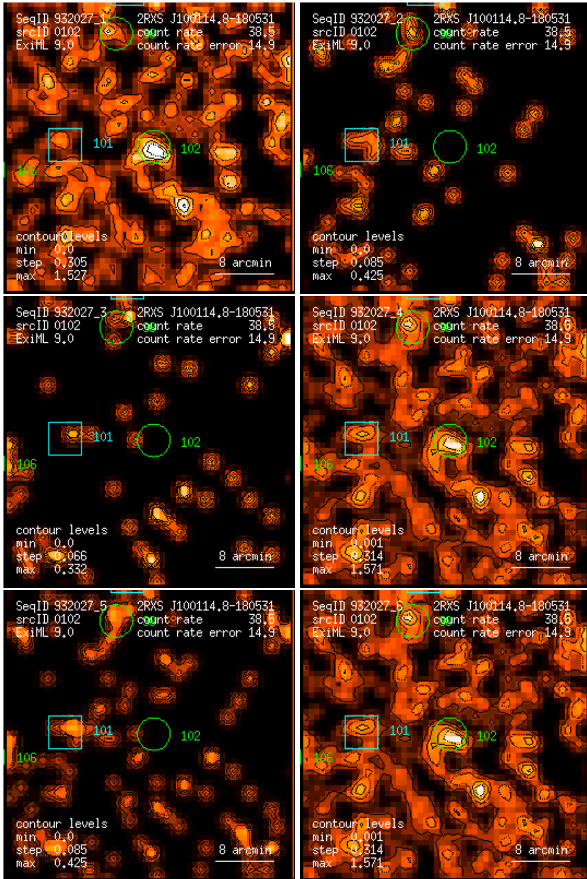
Figure 102: RASS 932027: detection 0102: band rate images, Gaussian filter: (1) PSPC channels 11 – 41, (2) 52 – 90, (3) 91 – 201, (4) 11 – 235, (5) 52 – 201, (6) 11 – 201. Broad band rates in counts/ks. Band rate contour levels in counts/ks/arcmin 2 .
