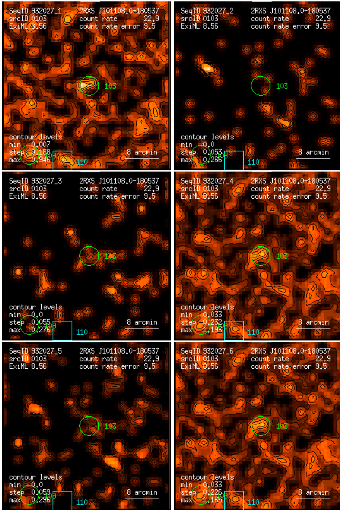
Figure 103: RASS 932027: detection 0103: band rate images, Gaussian filter: (1) PSPC channels 11 – 41, (2) 52 – 90, (3) 91 – 201, (4) 11 – 235, (5) 52 – 201, (6) 11 – 201. Broad band rates in counts/ks. Band rate contour levels in counts/ks/arcmin 2 .
