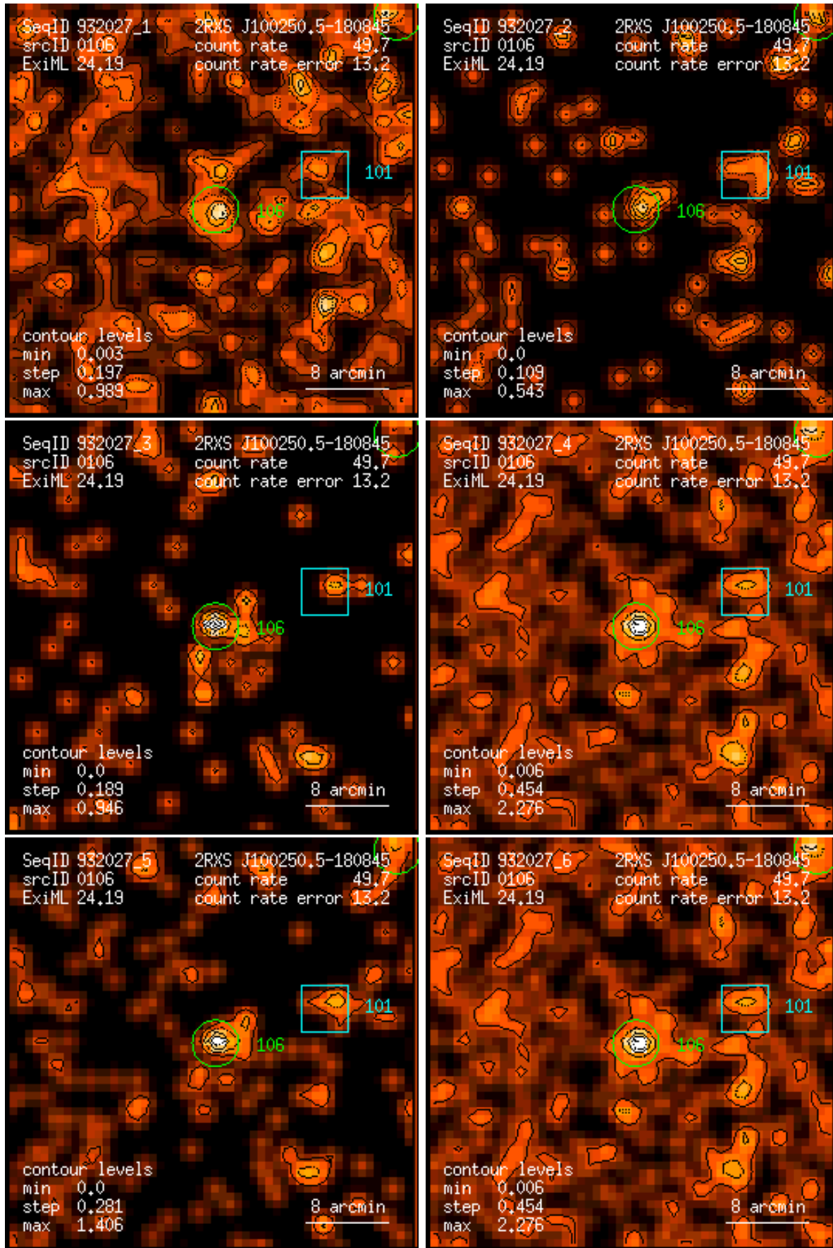
Figure 106: RASS 932027: detection 0106: band rate images, Gaussian filter: (1) PSPC channels 11 – 41, (2) 52 – 90, (3) 91 – 201, (4) 11 – 235, (5) 52 – 201, (6) 11 – 201. Broad band rates in counts/ks. Band rate contour levels in counts/ks/arcmin 2 .
