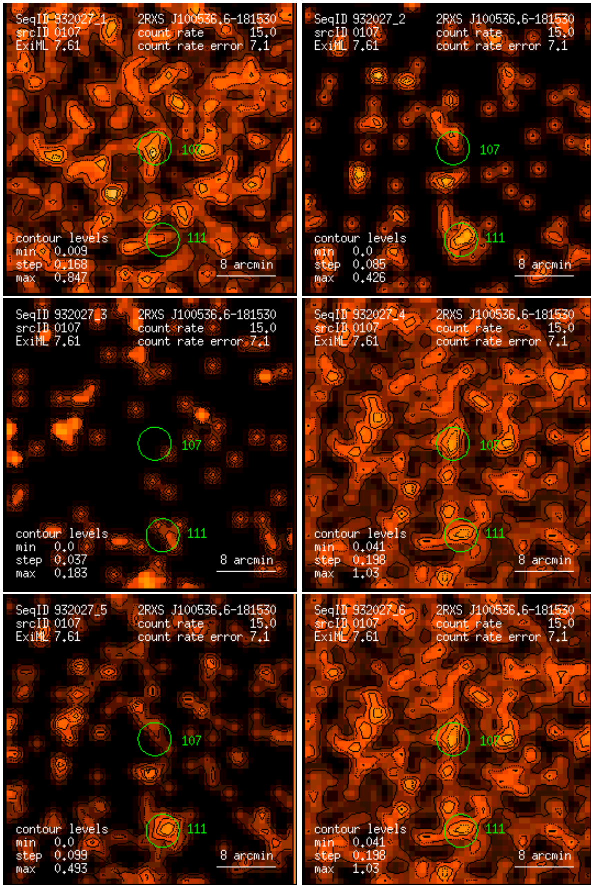
Figure 107: RASS 932027: detection 0107: band rate images, Gaussian filter: (1) PSPC channels 11 – 41, (2) 52 – 90, (3) 91 – 201, (4) 11 – 235, (5) 52 – 201, (6) 11 – 201. Broad band rates in counts/ks. Band rate contour levels in counts/ks/arcmin 2 .
