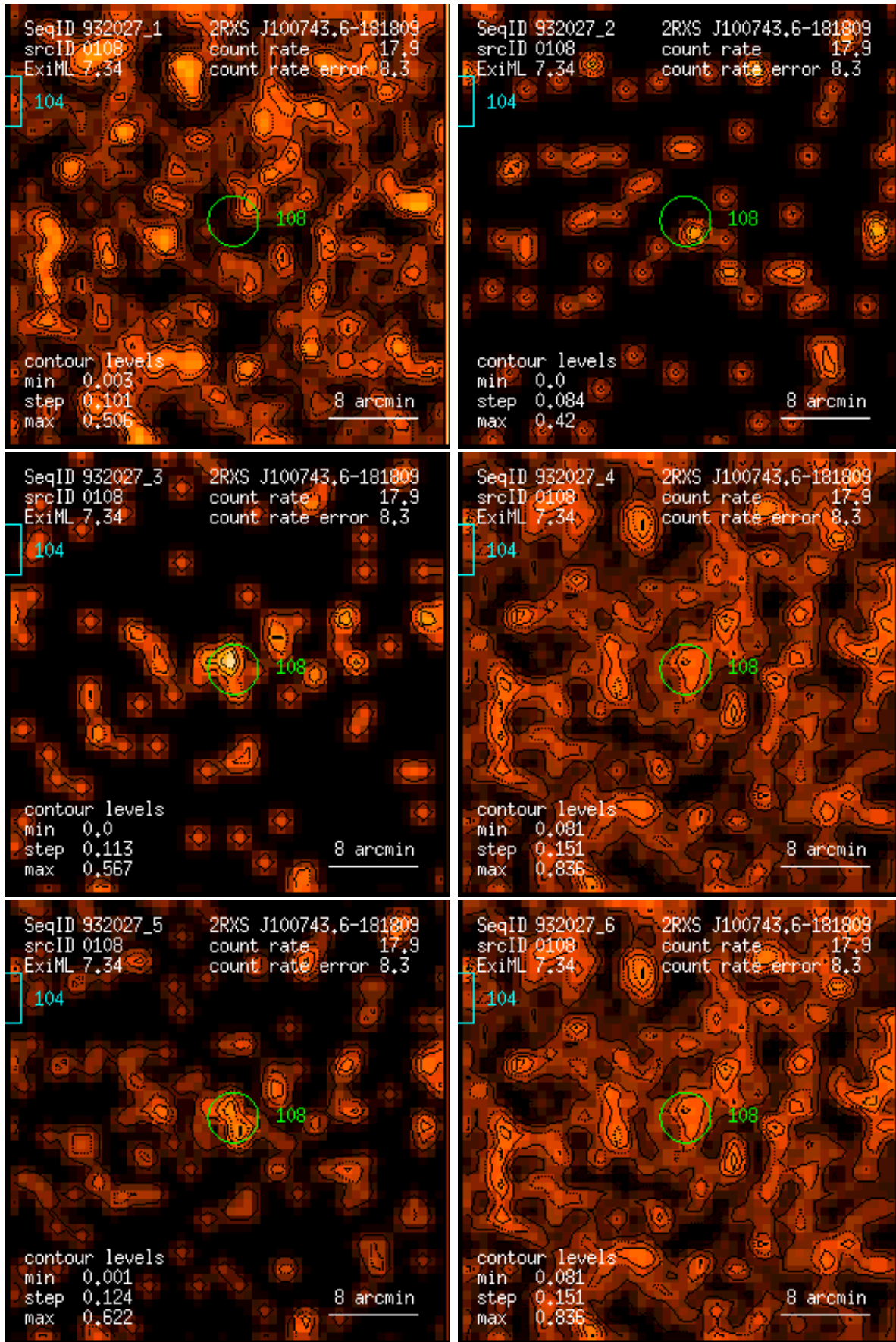
Figure 108: RASS 932027: detection 0108: band rate images, Gaussian filter: (1) PSPC channels 11 – 41, (2) 52 – 90, (3) 91 – 201, (4) 11 – 235, (5) 52 – 201, (6) 11 – 201. Broad band rates in counts/ks. Band rate contour levels in counts/ks/arcmin 2 .
