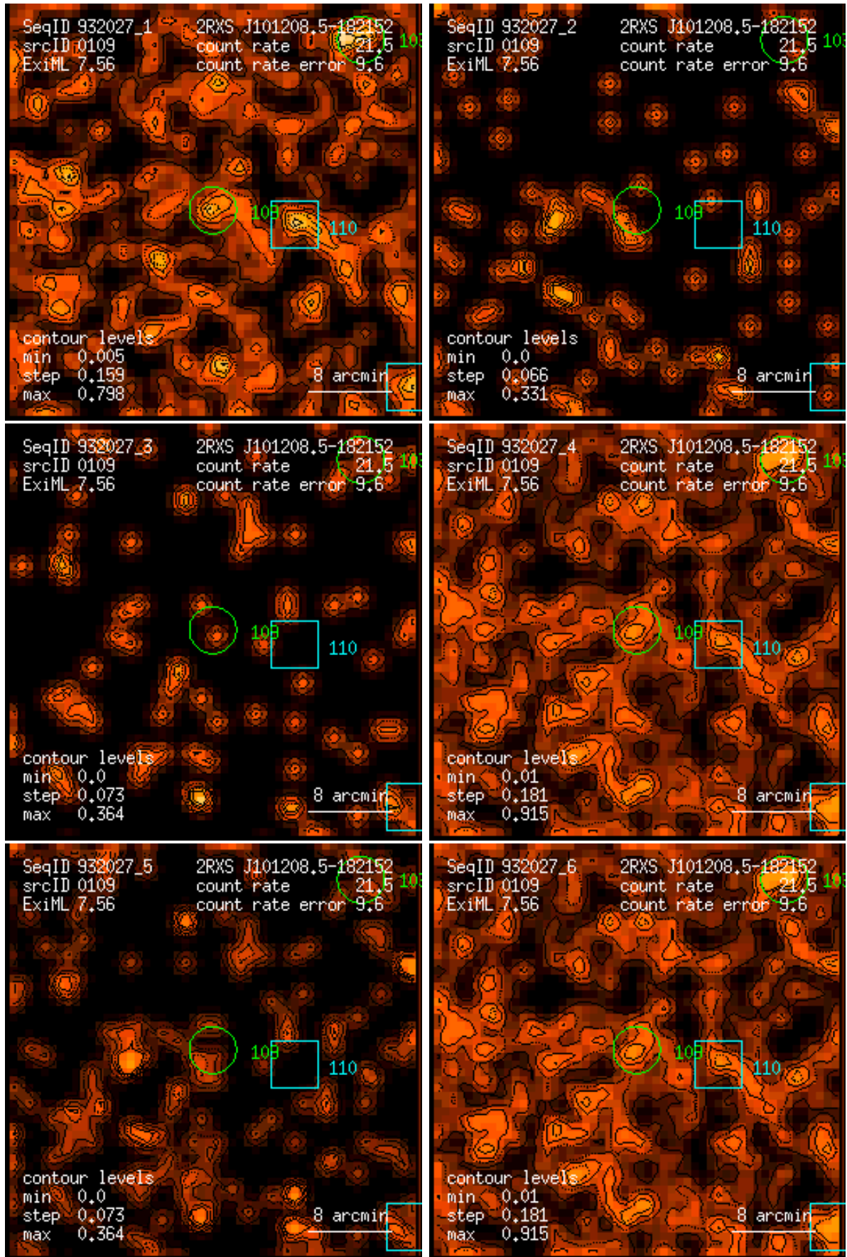
Figure 109: RASS 932027: detection 0109: band rate images, Gaussian filter: (1) PSPC channels 11 – 41, (2) 52 – 90, (3) 91 – 201, (4) 11 – 235, (5) 52 – 201, (6) 11 – 201. Broad band rates in counts/ks. Band rate contour levels in counts/ks/arcmin 2 .
