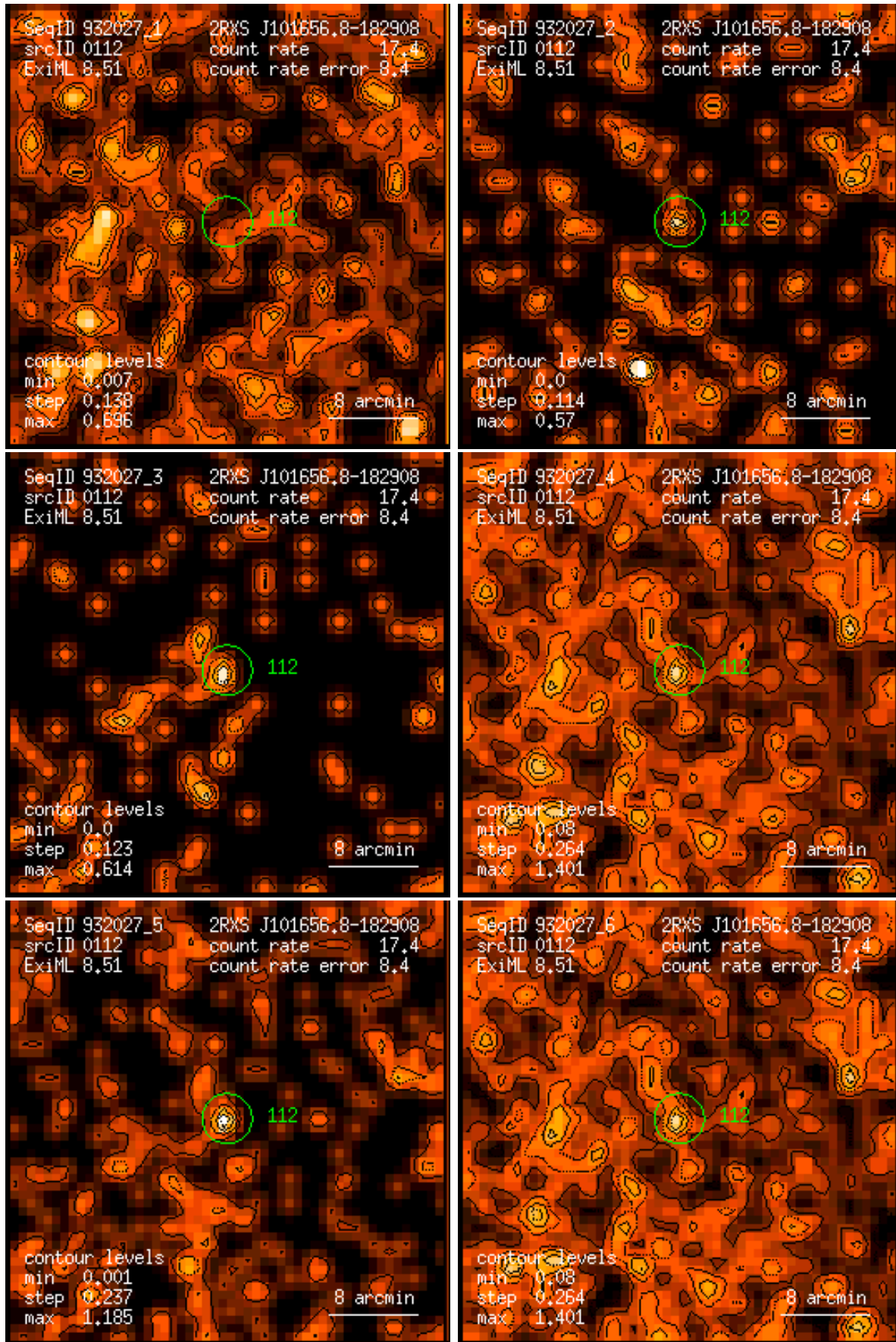
Figure 112: RASS 932027: detection 0112: band rate images, Gaussian filter: (1) PSPC channels 11 – 41, (2) 52 – 90, (3) 91 – 201, (4) 11 – 235, (5) 52 – 201, (6) 11 – 201. Broad band rates in counts/ks. Band rate contour levels in counts/ks/arcmin 2 .
