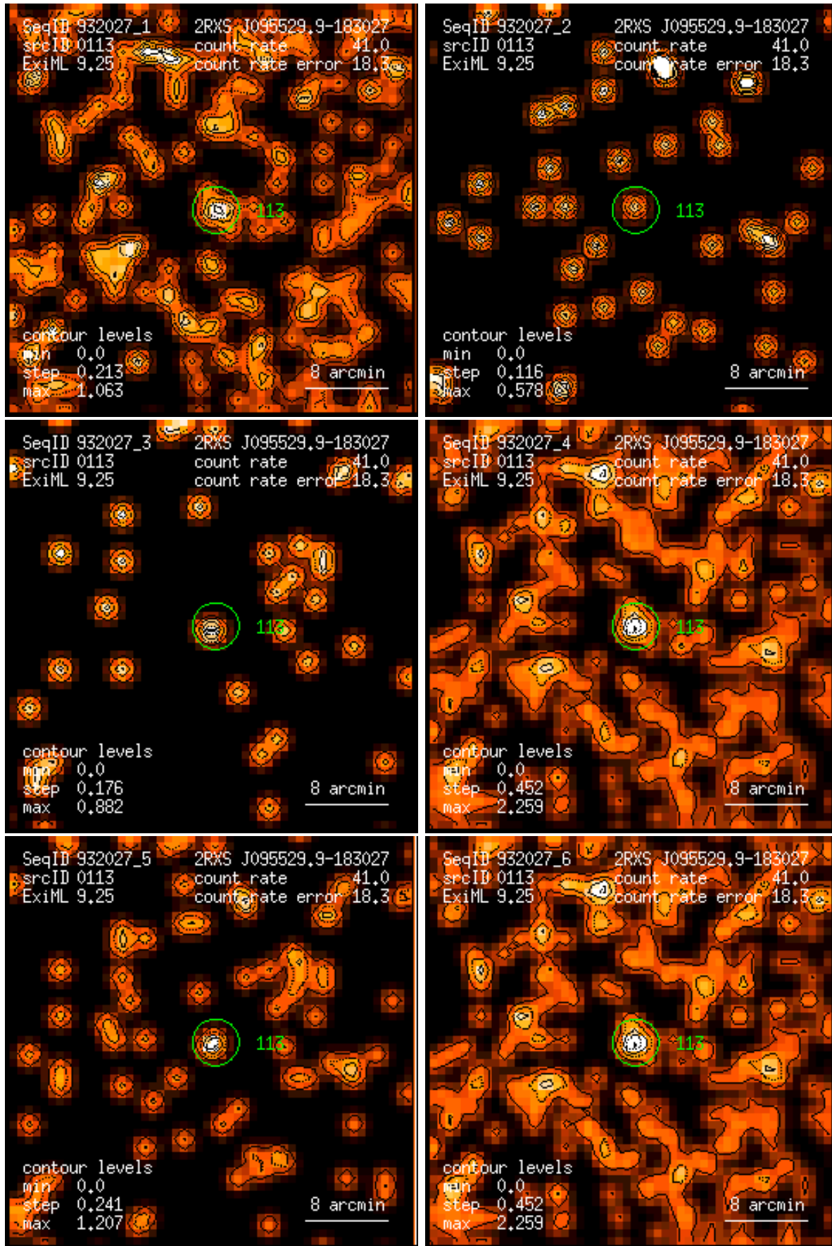
Figure 113: RASS 932027: detection 0113: band rate images, Gaussian filter: (1) PSPC channels 11 – 41, (2) 52 – 90, (3) 91 – 201, (4) 11 – 235, (5) 52 – 201, (6) 11 – 201. Broad band rates in counts/ks. Band rate contour levels in counts/ks/arcmin 2 .
