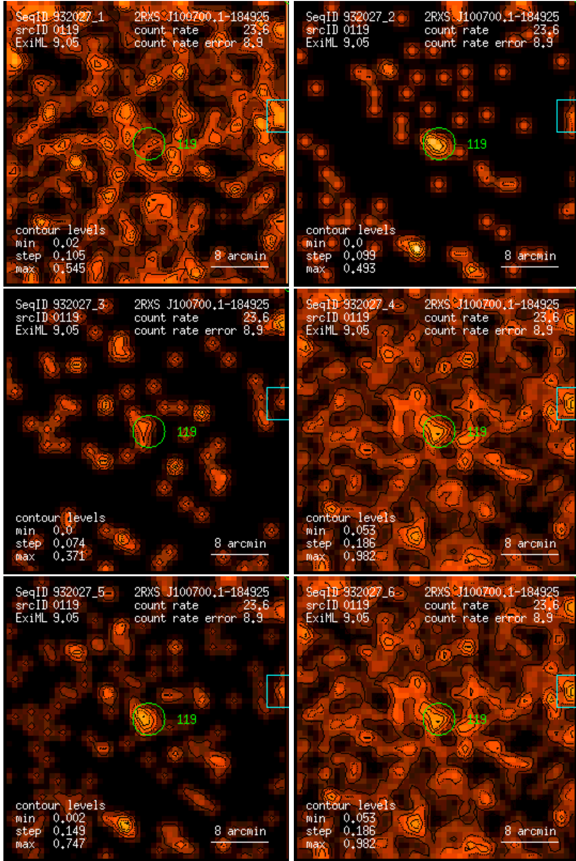
Figure 119: RASS 932027: detection 0119: band rate images, Gaussian filter: (1) PSPC channels 11 – 41, (2) 52 – 90, (3) 91 – 201, (4) 11 – 235, (5) 52 – 201, (6) 11 – 201. Broad band rates in counts/ks. Band rate contour levels in counts/ks/arcmin 2 .
