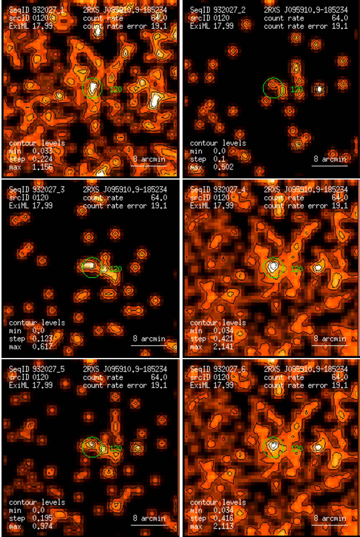
Figure 120: RASS 932027: detection 0120: band rate images, Gaussian filter: (1) PSPC channels 11 – 41, (2) 52 – 90, (3) 91 – 201, (4) 11 – 235, (5) 52 – 201, (6) 11 – 201. Broad band rates in counts/ks. Band rate contour levels in counts/ks/arcmin 2 .
