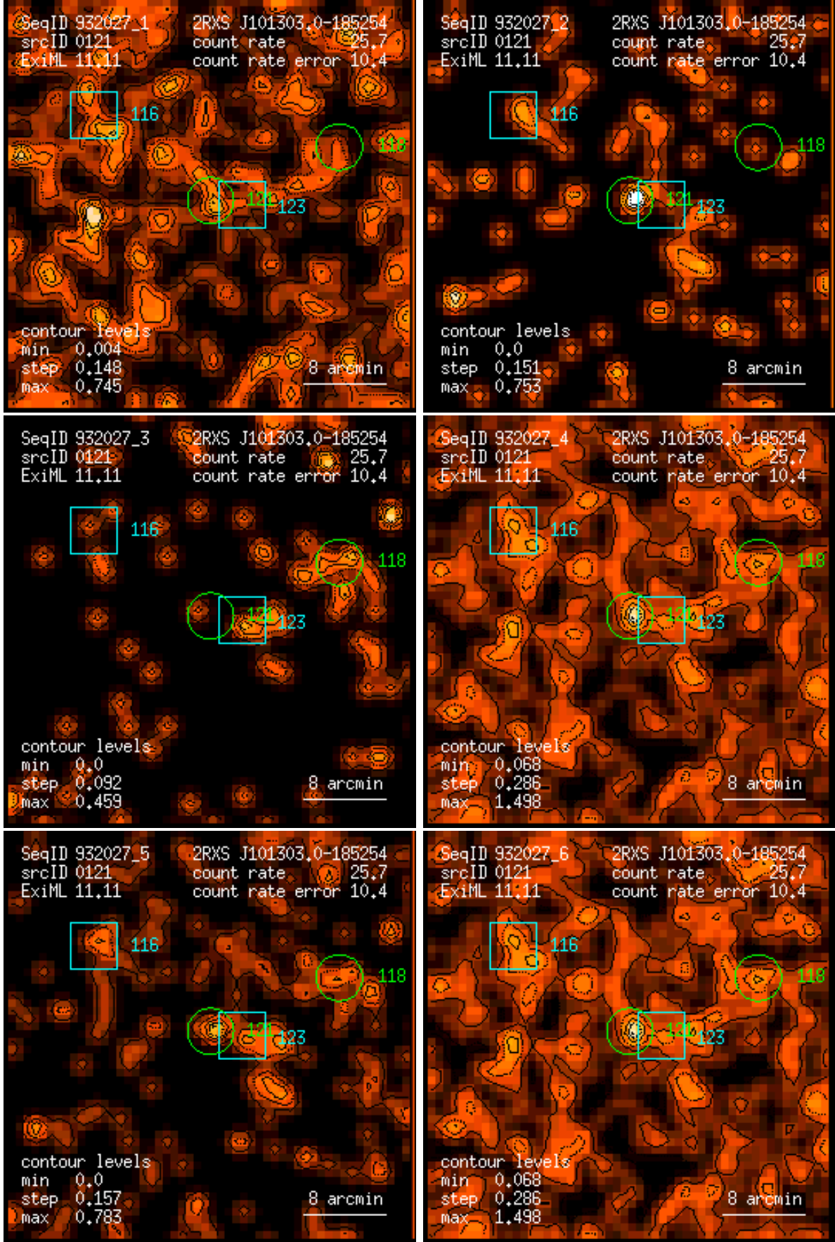
Figure 121: RASS 932027: detection 0121: band rate images, Gaussian filter: (1) PSPC channels 11 – 41, (2) 52 – 90, (3) 91 – 201, (4) 11 – 235, (5) 52 – 201, (6) 11 – 201. Broad band rates in counts/ks. Band rate contour levels in counts/ks/arcmin 2 .
