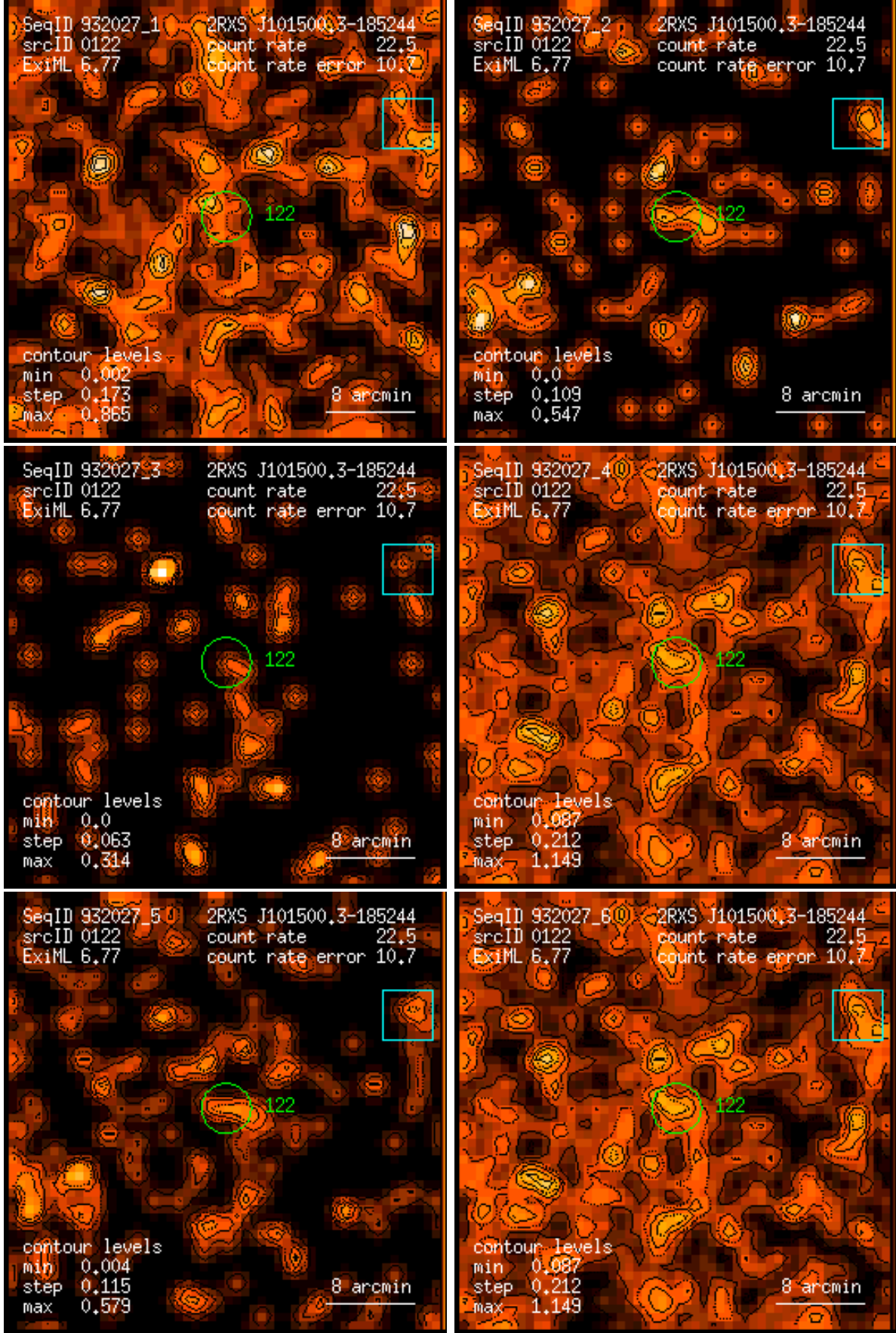
Figure 122: RASS 932027: detection 0122: band rate images, Gaussian filter: (1) PSPC channels 11 – 41, (2) 52 – 90, (3) 91 – 201, (4) 11 – 235, (5) 52 – 201, (6) 11 – 201. Broad band rates in counts/ks. Band rate contour levels in counts/ks/arcmin 2 .
