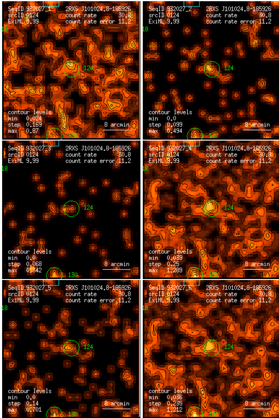
Figure 124: RASS 932027: detection 0124: band rate images, Gaussian filter: (1) PSPC channels 11 – 41, (2) 52 – 90, (3) 91 – 201, (4) 11 – 235, (5) 52 – 201, (6) 11 – 201. Broad band rates in counts/ks. Band rate contour levels in counts/ks/arcmin 2 .
