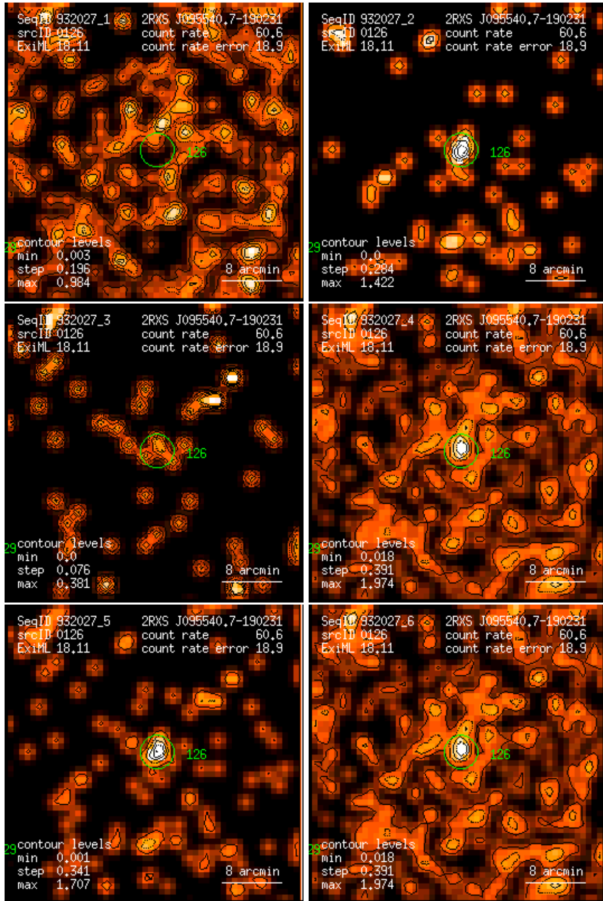
Figure 126: RASS 932027: detection 0126: band rate images, Gaussian filter: (1) PSPC channels 11 – 41, (2) 52 – 90, (3) 91 – 201, (4) 11 – 235, (5) 52 – 201, (6) 11 – 201. Broad band rates in counts/ks. Band rate contour levels in counts/ks/arcmin 2 .
