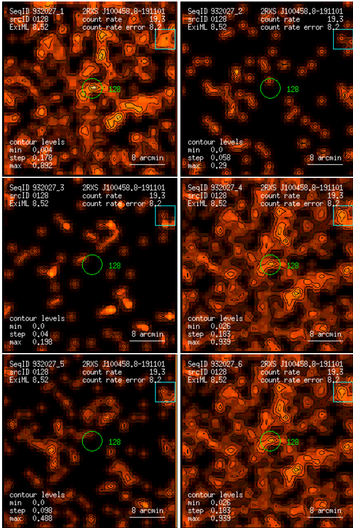
Figure 128: RASS 932027: detection 0128: band rate images, Gaussian filter: (1) PSPC channels 11 – 41, (2) 52 – 90, (3) 91 – 201, (4) 11 – 235, (5) 52 – 201, (6) 11 – 201. Broad band rates in counts/ks. Band rate contour levels in counts/ks/arcmin 2 .
