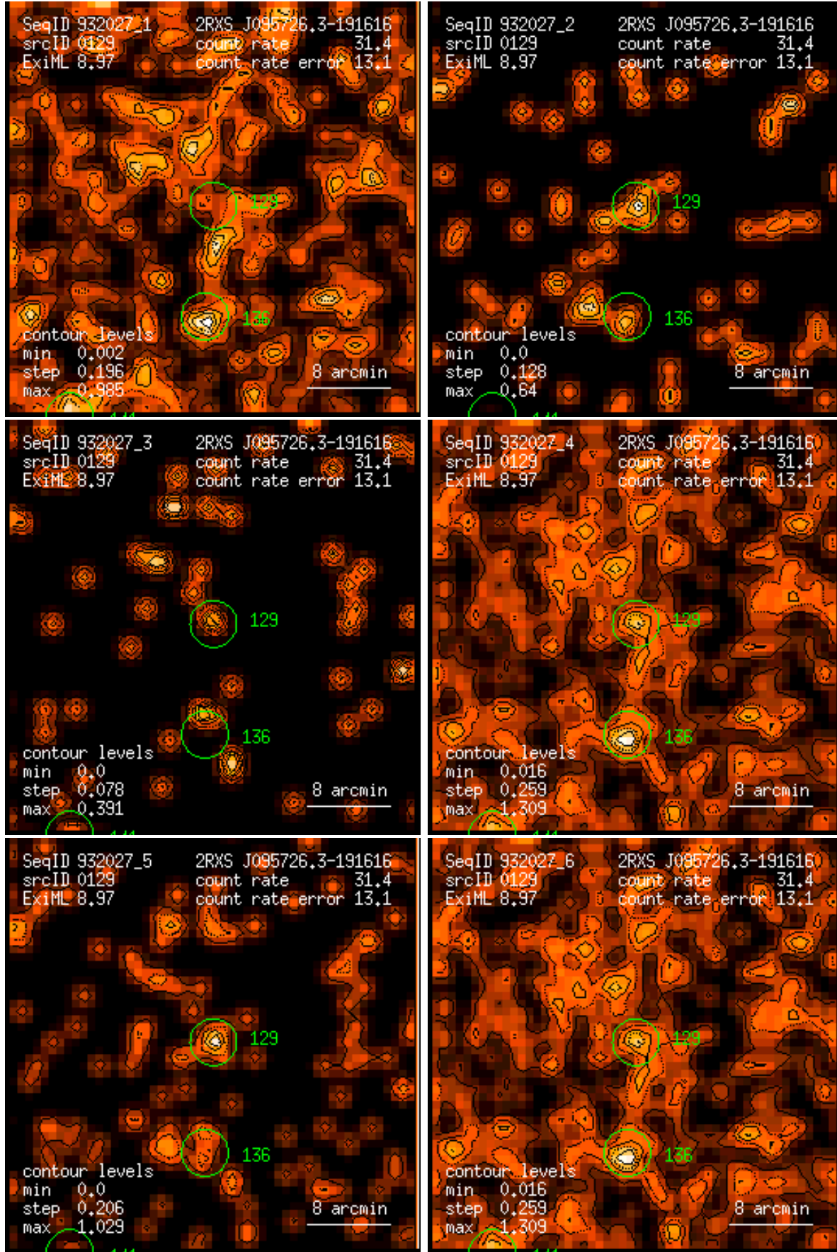
Figure 129: RASS 932027: detection 0129: band rate images, Gaussian filter: (1) PSPC channels 11 – 41, (2) 52 – 90, (3) 91 – 201, (4) 11 – 235, (5) 52 – 201, (6) 11 – 201. Broad band rates in counts/ks. Band rate contour levels in counts/ks/arcmin 2 .
